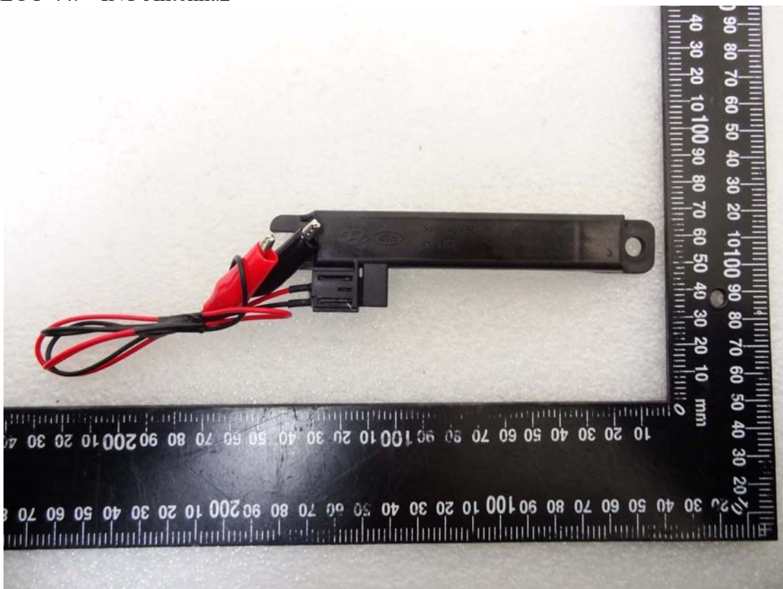
EUT-44. INT Antenna2
