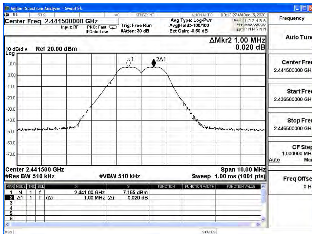
Channel 39
