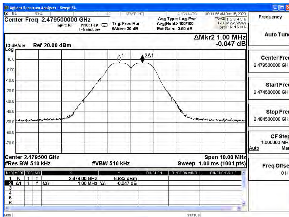
Channel 78
