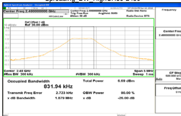
Spreading BW HighCH39-2480
