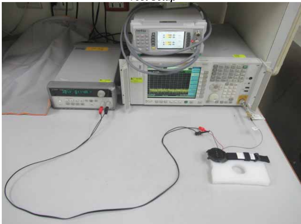
Test Setup
