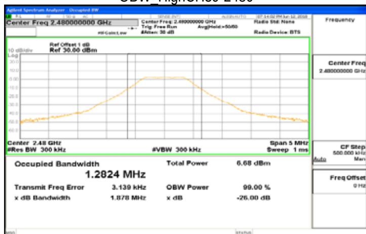
OBW HighCH39-2480
