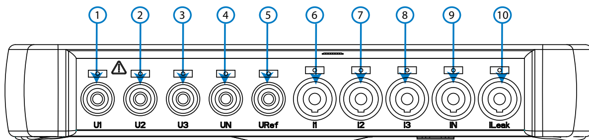
Figure 12: Bornes MYeBOX 1500, face inférieure
