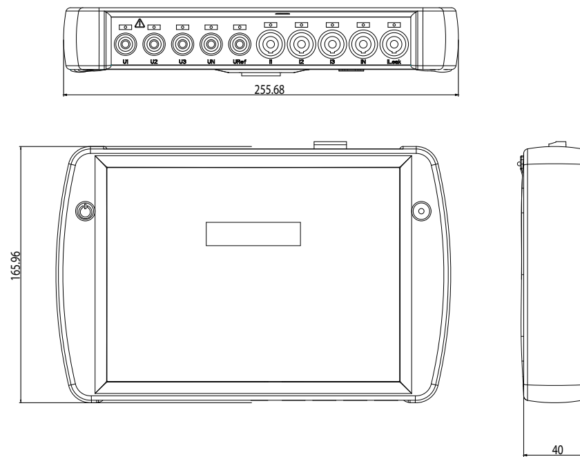
Figure 58: Dimensions MYeBOX.
