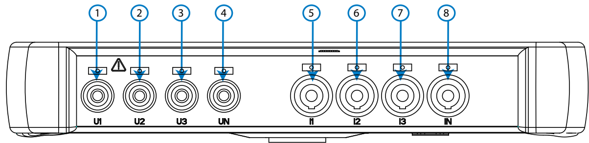
Figure 10: Bornes MYeBOX 150, face inférieure
