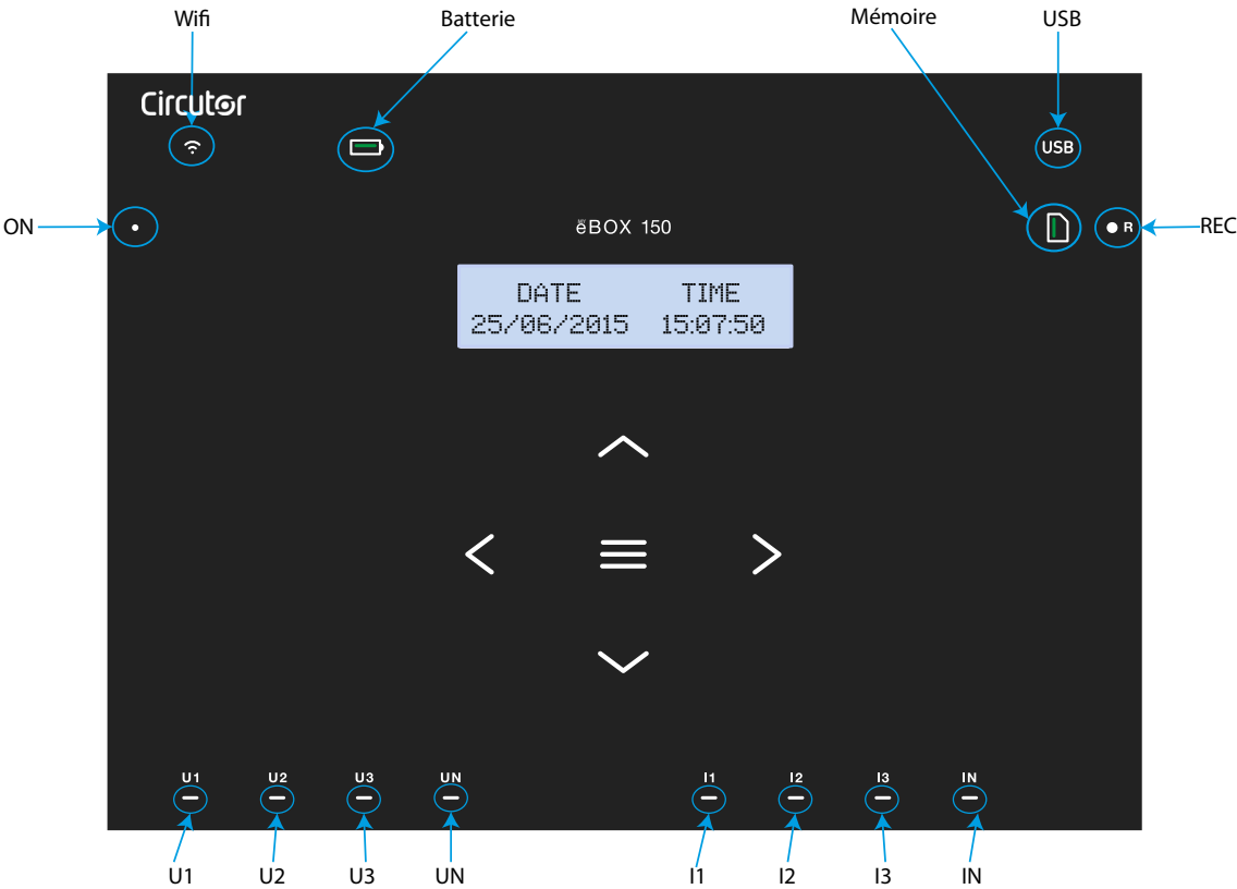
Figure 34: Indicateurs DEL MYeBOX 150.
