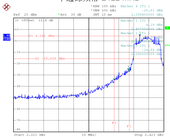
下邊緣頻帶-2412 MHz
