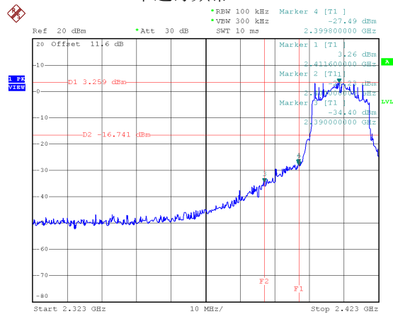
下邊緣頻帶-2412 MHz
