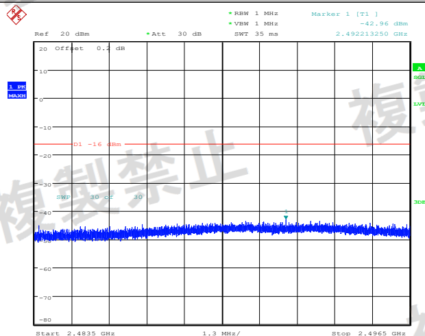
NTNV_11B_Ant1_2412_2483.5~2496.5
