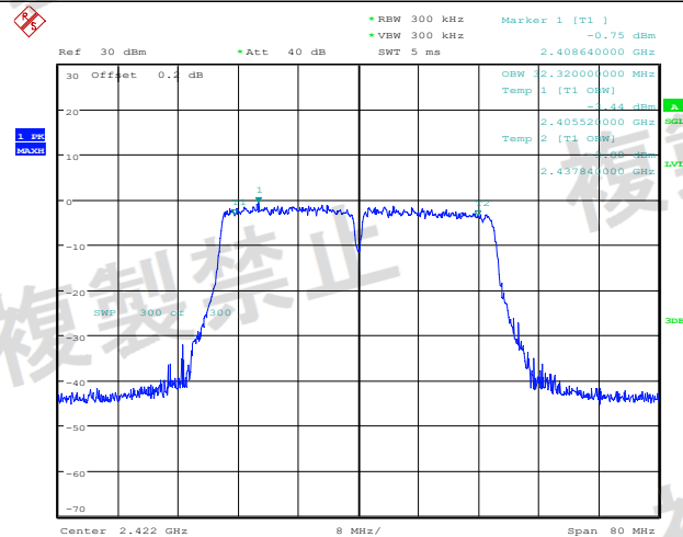
NTNV_11N40SISO_Ant1_2422
