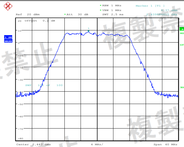
NTNV_11G_Ant1_2442
