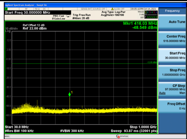
CH39 (2480MHz) LE(1Mbps)
