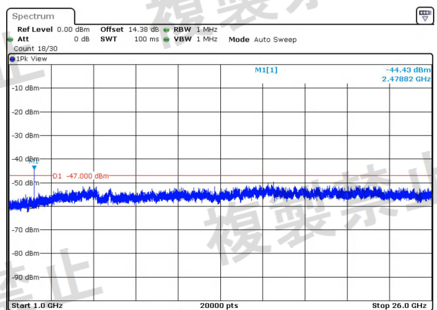
NTNV-11AC40MIMO-Ant2-5710-1000~26000-See table
