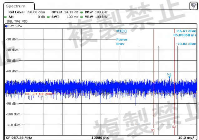
NTNV-11N20-Ant2-5600-30~1000-PASS
