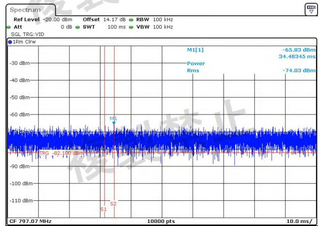
NTNV-11A-Ant2-5600-30~1000-PASS
