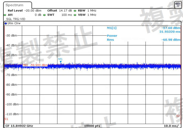
NTNV-11A-Ant2-5600-1000~26000-PASS
