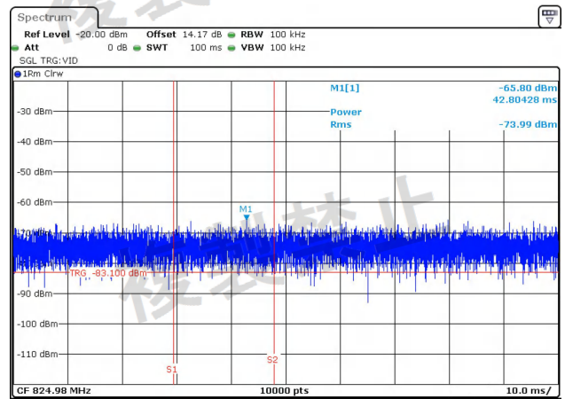
NTNV-11N20-Ant2-5600-30~1000-PASS
