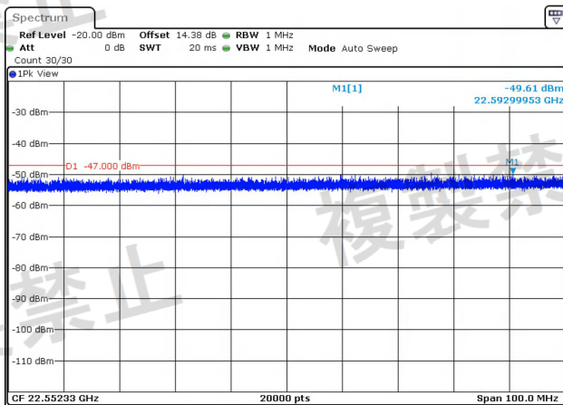
NTNV-11A-Ant2-5720-1000~26000-PASS
