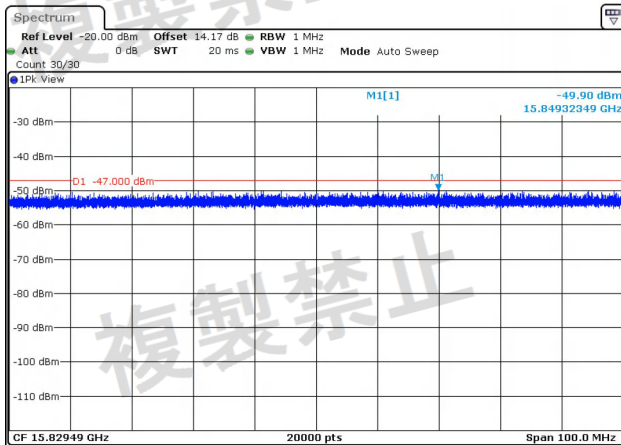
NTNV-11A-Ant2-5600-1000~26000-PASS
