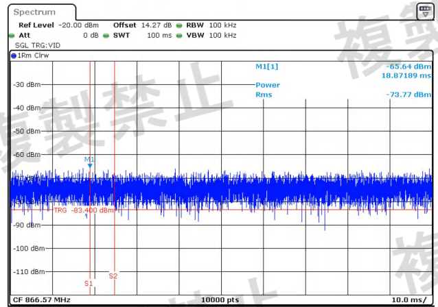
NTNV-11N20-Ant2-5500-30~1000-PASS
