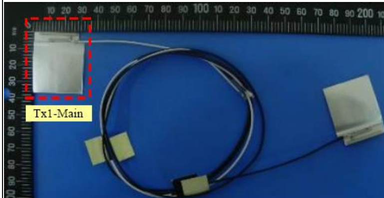
Antenna 12 F.0G.FN-6025-001(Main), F.0G.FN-6025-001(Aux), Speed, 2016/12/21
