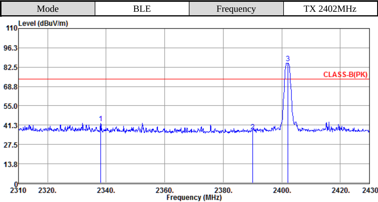
Antenna at Horizontal Polarization
