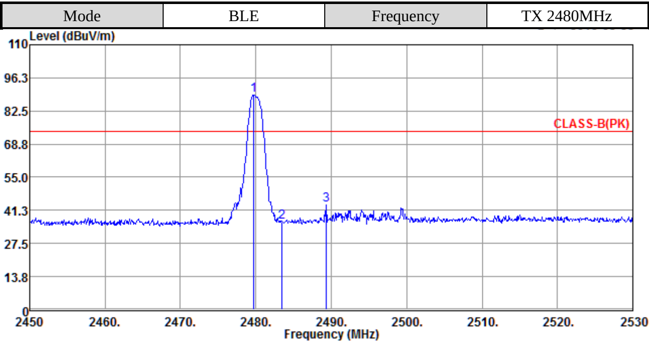
Antenna at Vertical Polarization
