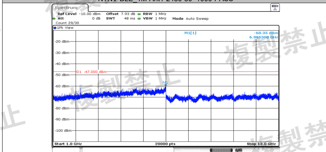
NTNV-BLE_1M-Ant1-2480-1000~13000-PASS
