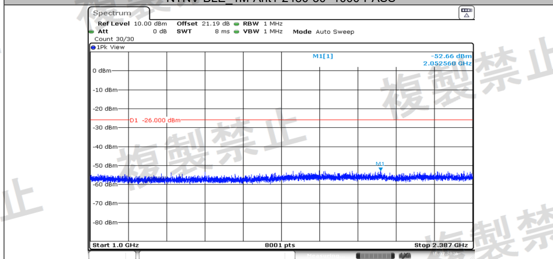
NTNV-BLE 1M-Ant1-2480-1000~2387-PASS
