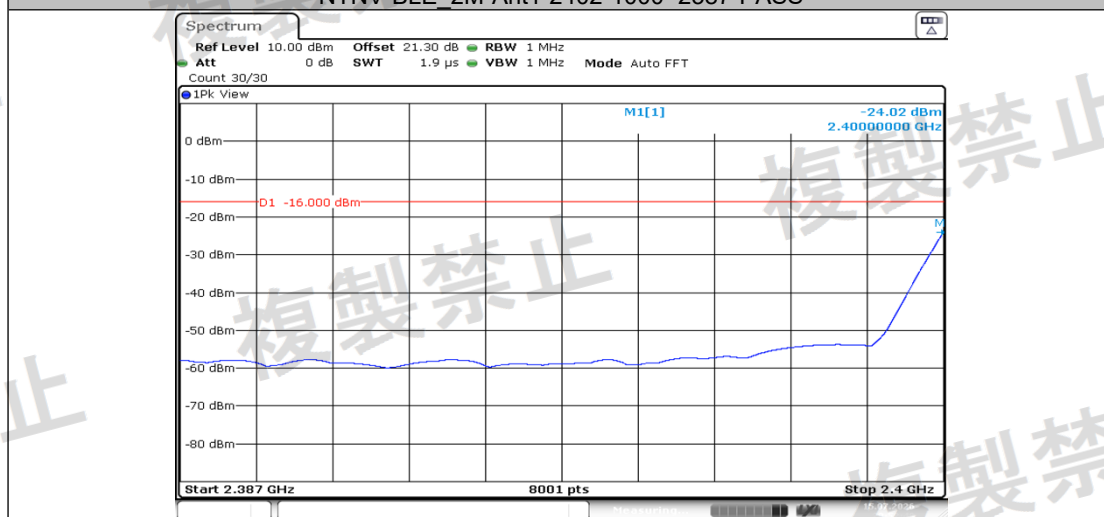
NTNV-BLE_2M-Ant1-2402-2387~2400-PASS
