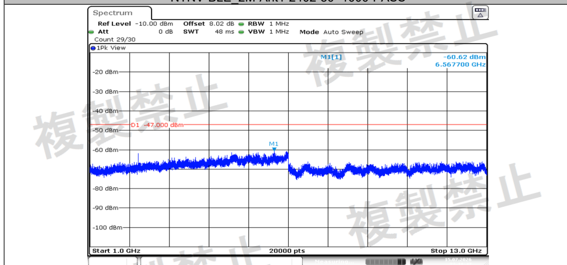
NTNV-BLE_2M-Ant1-2402-1000~13000-PASS
