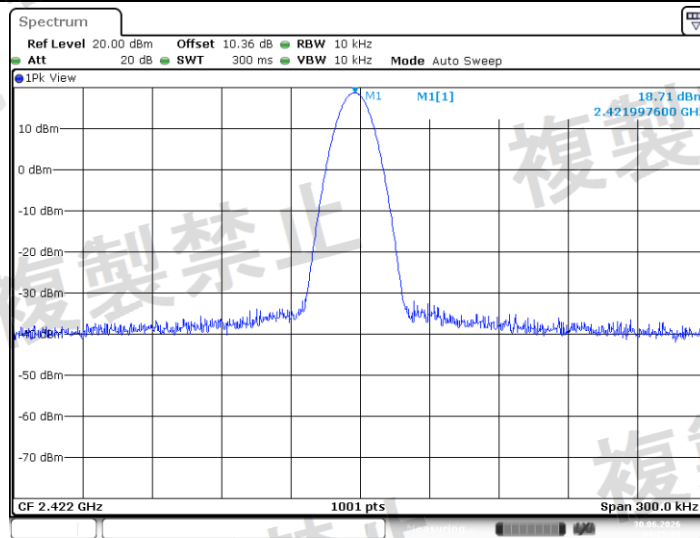
NTNV_11N40SISO_Ant1_2422
