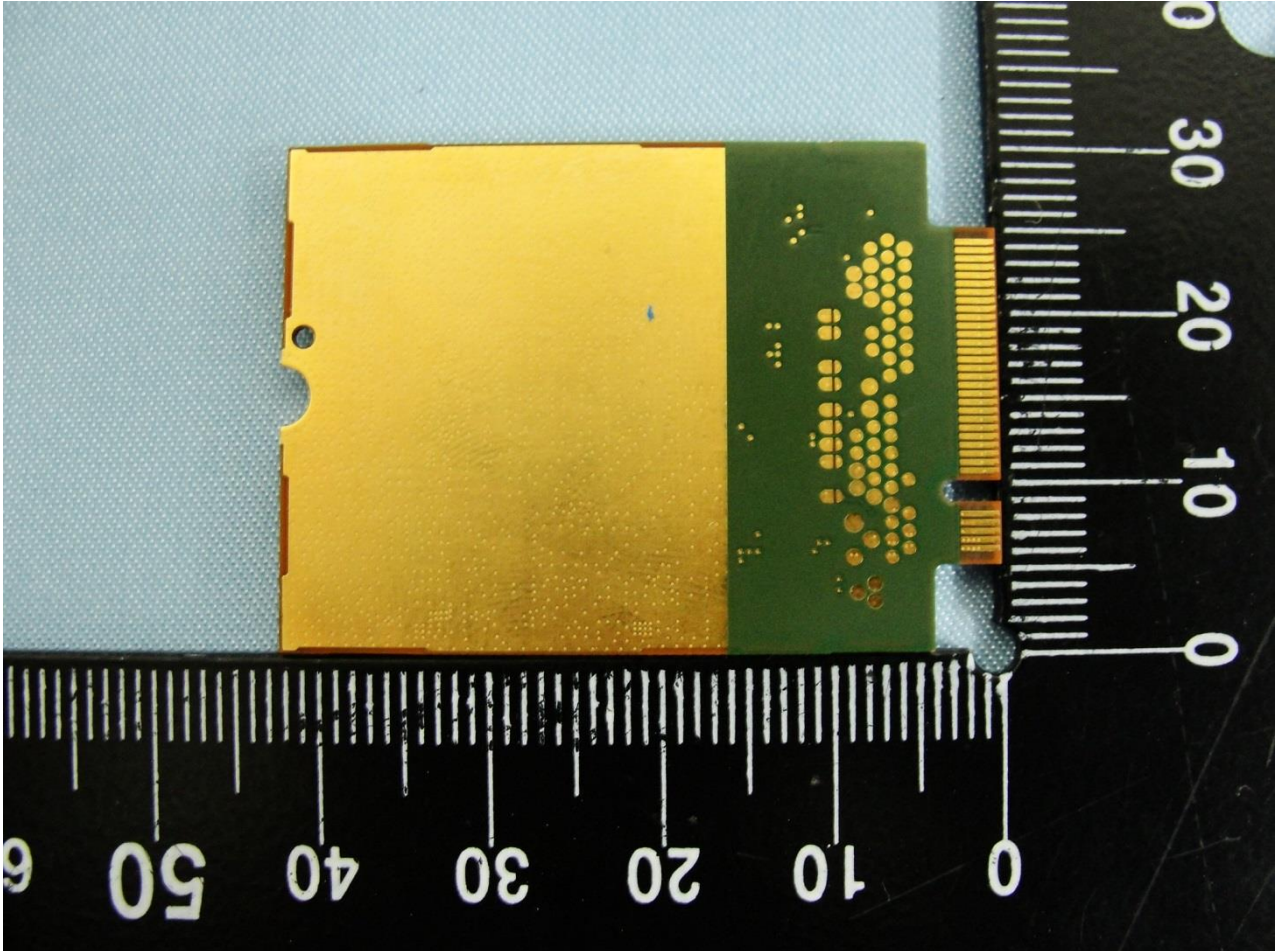
EUT: Wireless Module (Brand Name: AirPrime / Model Name: EM7455)
