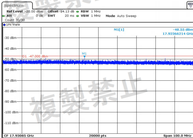
NTNV-11AC40MIMO-Ant1-5590-1000~26000-PASS
