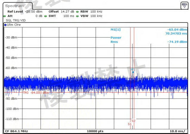
NTNV-11AC40MIMO-Ant2-5510-30~1000-PASS
