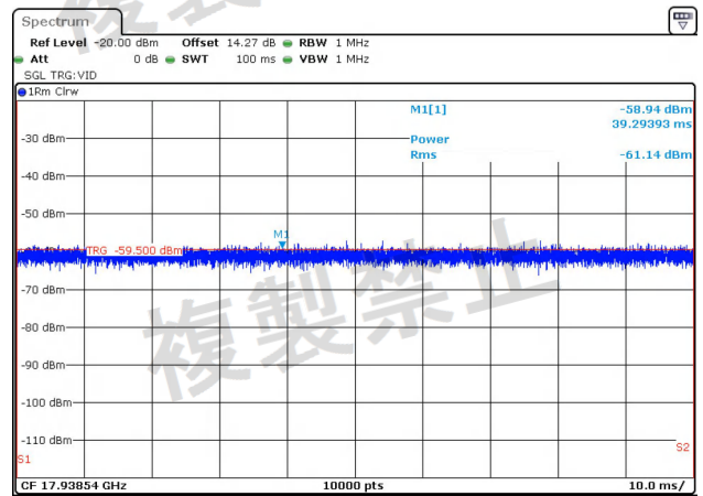
NTNV-11AC40-Ant2-5510-1000~26000-PASS
