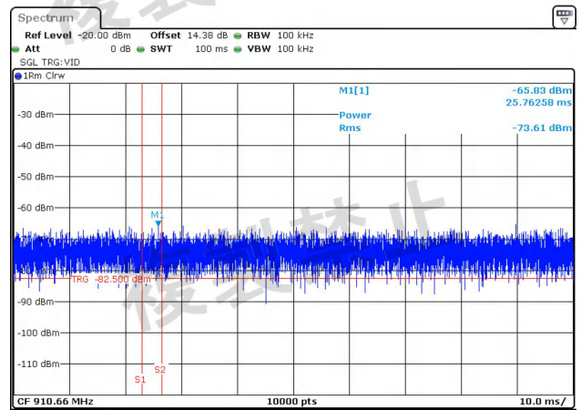
NTNV-11AC40MIMO-Ant1-5710-30~1000-PASS
