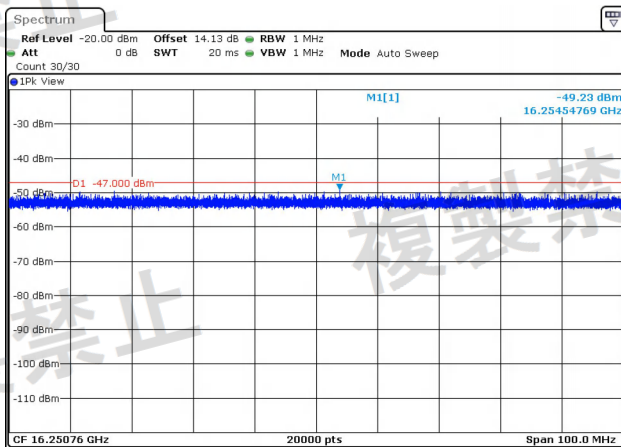
NTNV-11AC20MIMO-Ant2-5600-1000~26000-PASS
