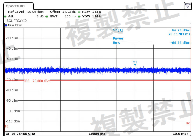
NTNV-11AC20MIMO-Ant2-5600-1000~26000-PASS
