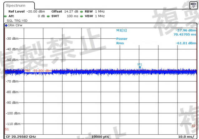
NTNV-11AC40MIMO-Ant2-5510-1000~26000-PASS
