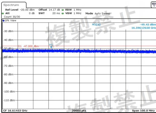
NTNV-11AC20MIMO-Ant2-5600-1000~26000-PASS
