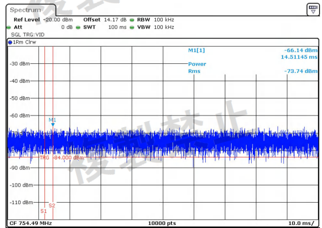
NTNV-11AC40MIMO-Ant2-5590-30~1000-PASS
