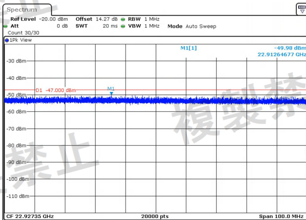
NTNV-11AC40-Ant2-5510-1000~26000-PASS
