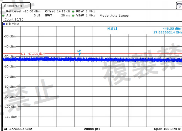
NTNV-11AC40MIMO-Ant2-5590-1000~26000-PASS
