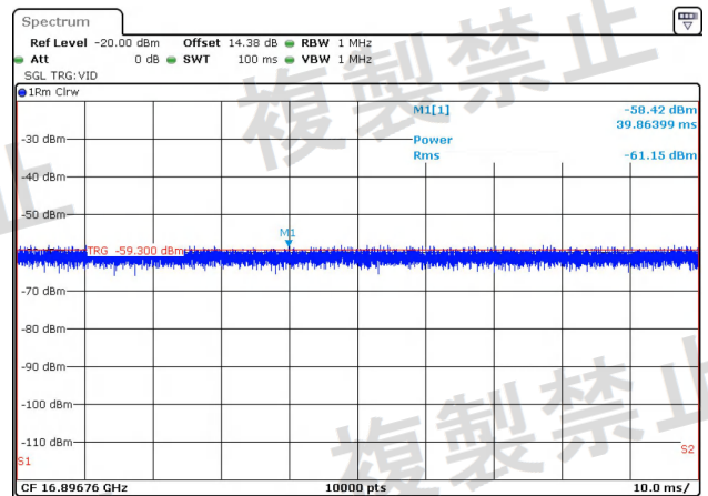
NTNV-11AC20-Ant2-5720-1000~26000-PASS
