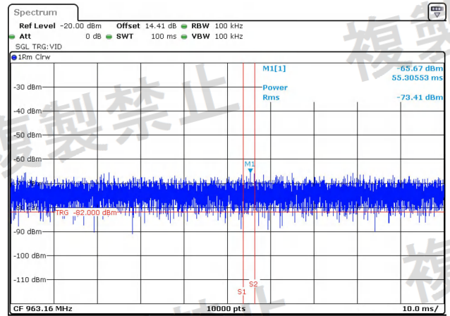
NTNV-11AC40MIMO-Ant2-5710-30~1000-PASS
