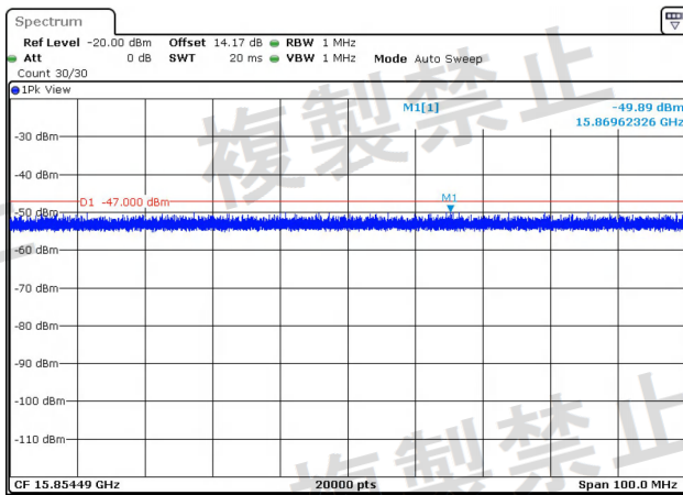
NTNV-11AC40MIMO-Ant2-5590-1000~26000-PASS
