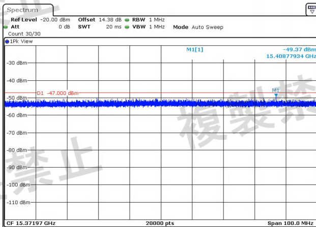
NTNV-11AC20MIMO-Ant2-5720-1000~26000-PASS
