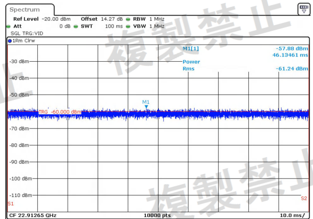
NTNV-11AC40-Ant2-5510-1000~26000-PASS
