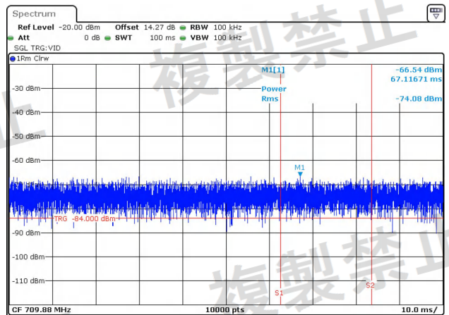
NTNV-11AC40MIMO-Ant2-5510-30~1000-PASS
