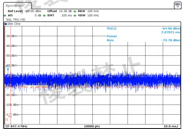
NTNV-11AC20MIMO-Ant1-5720-30~1000-PASS
