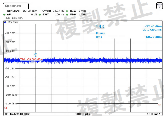
NTNV-11AC20MIMO-Ant1-5600-1000~26000-PASS
