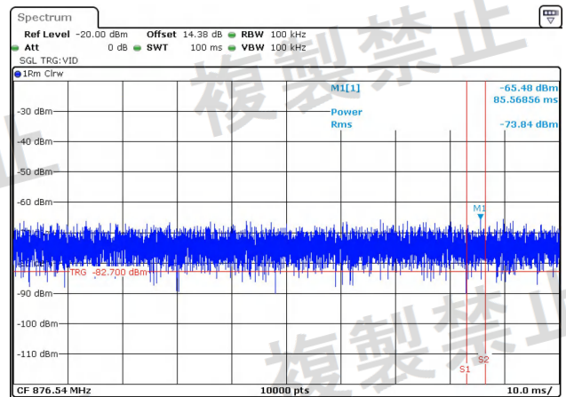
NTNV-11AC40-Ant2-5710-30~1000-PASS
