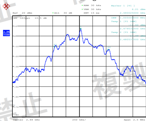
2.4G SRD_High Channel
