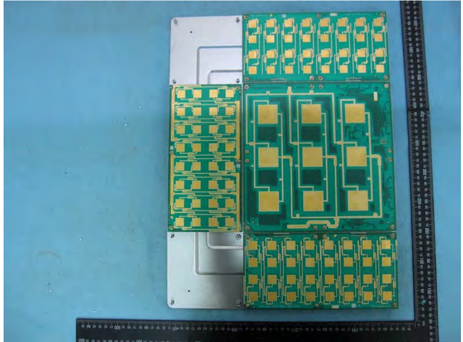
Ant. Set 1: Directional Antenna
