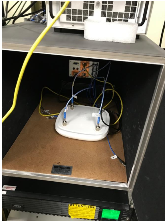
Title: Radio Conducted Test Setup
