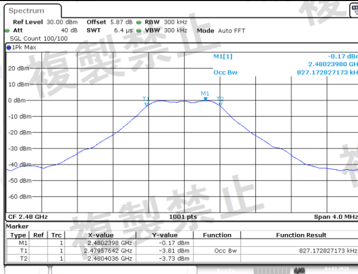
NTLV_BLE_1M_Ant1_2480
