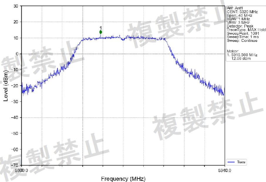
802.11ac(VHT20)_HCH_5320MHz_Ant1_NTNV
