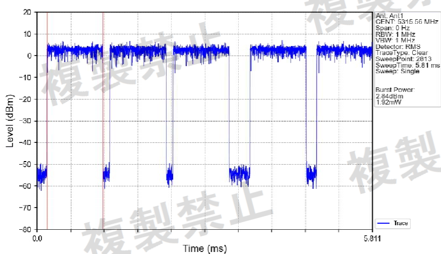
802.11ac(VHT20)_HCH_5320MHz_Ant1_NTNV
