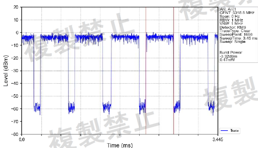
802.11ac(VHT40)_HCH_5310MHz_Ant1_NTNV
