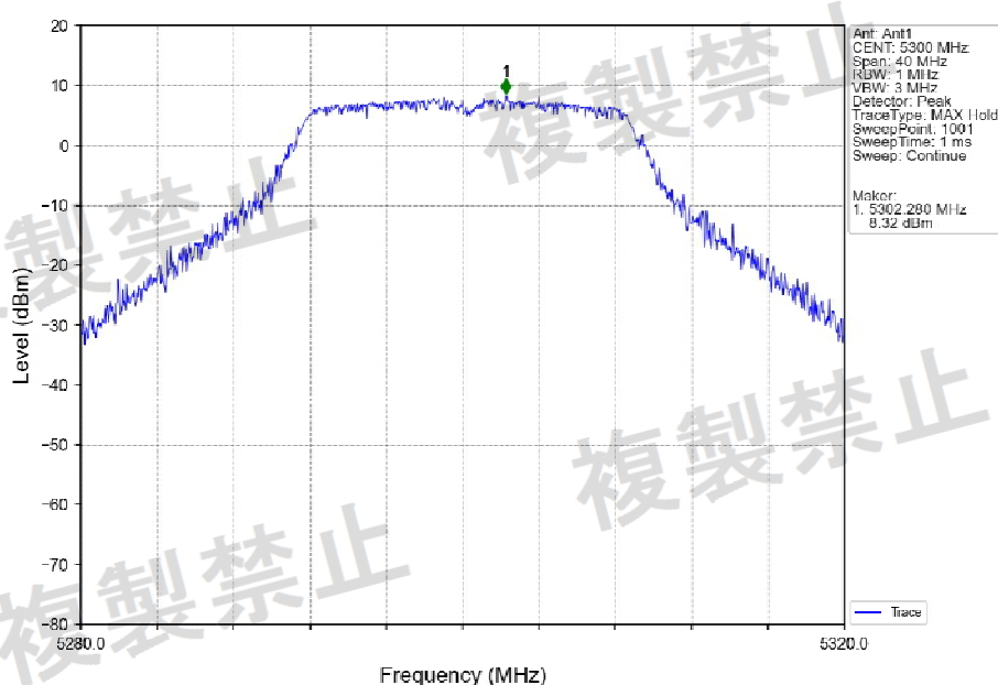
802.11ac(VHT20)_MCH_5300MHz_Ant1_NTNV
