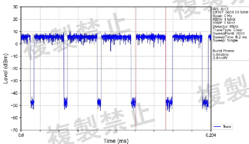
802.11ac(VHT20)_MCH_5600MHz_Ant1_NTNV
