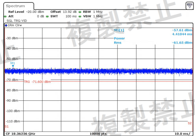
NTNV-11AC80MIMO-Ant2-5210-1000~26000-PASS
