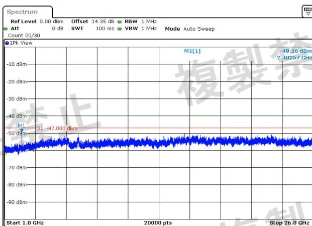
NTNV-11N20MIMO-Ant1-5320-1000~26000-See table below
