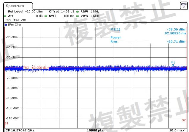
NTNV-11AC80MIMO-Ant1-5210-1000~26000-PASS
