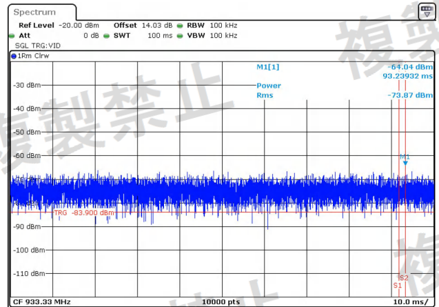
NTNV-11AC80MIMO-Ant2-5210-30~1000-PASS
