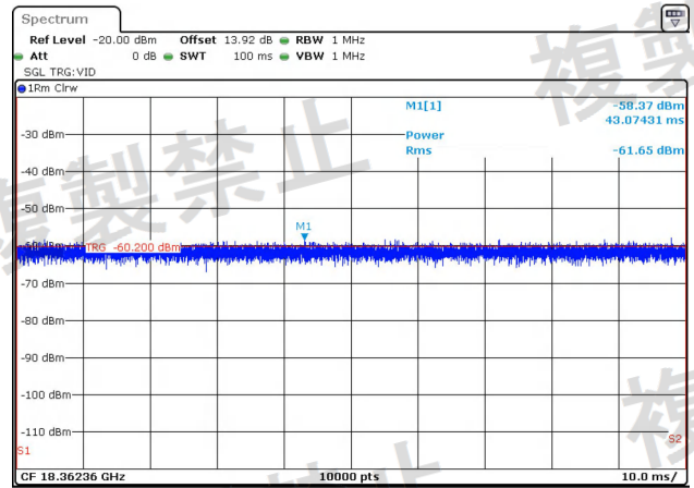
NTNV-11AC80MIMO-Ant1-5210-1000~26000-PASS
