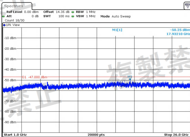
NTNV-11N20-Ant1-5320-1000~26000-See table below
