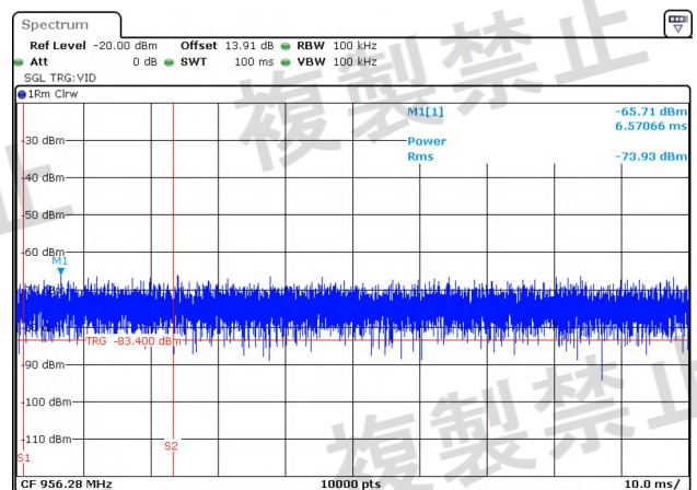
NTNV-11AC40MIMO-Ant1-5190-30~1000-PASS
