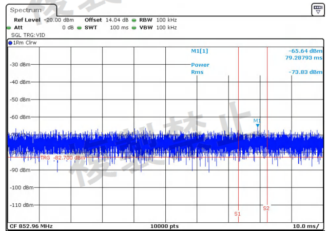
NTNV-11AC40MIMO-Ant2-5230-30~1000-PASS
