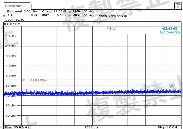
NTNV-11N20MIMO-Ant2-5300-30~1000-See table below
