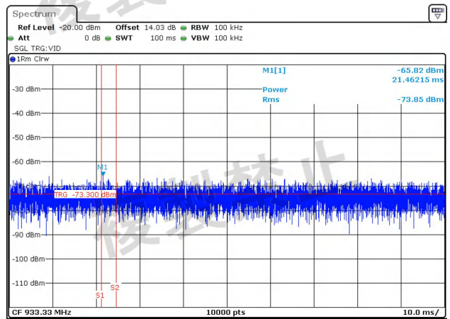
NTNV-11AC80MIMO-Ant2-5210-30~1000-PASS
