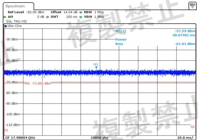
NTNV-11AC40MIMO-Ant2-5230-1000~26000-PASS
