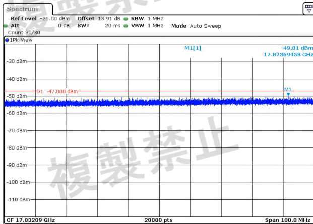
NTNV-11AC40MIMO-Ant2-5190-1000~26000-PASS
