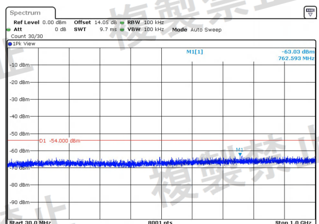
NTNV-11A-Ant2-5300-30~1000-See table below
