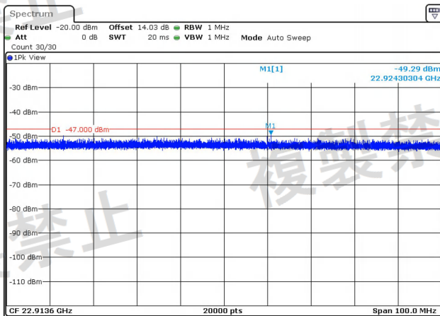
NTNV-11AC80-Ant1-5210-1000~26000-PASS
