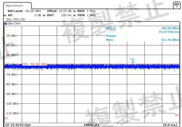
NTNV-11AC80-Ant1-5210-1000~26000-PASS
