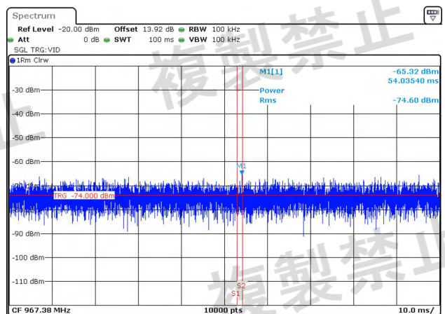
NTNV-11AC80MIMO-Ant2-5210-30~1000-PASS
