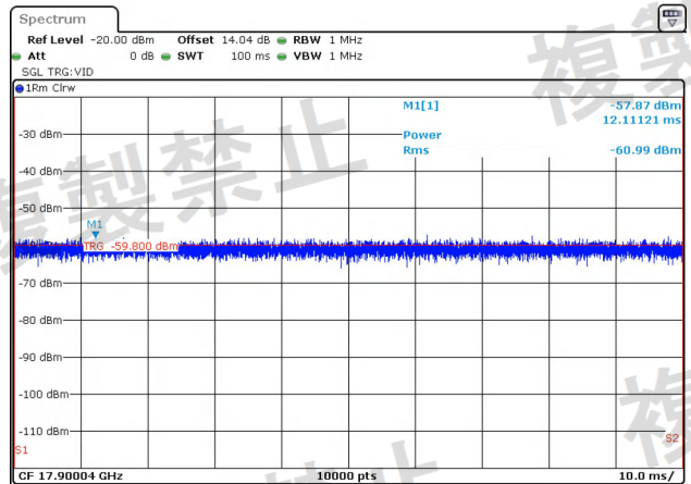
NTNV-11AC40MIMO-Ant1-5230-1000~26000-PASS
