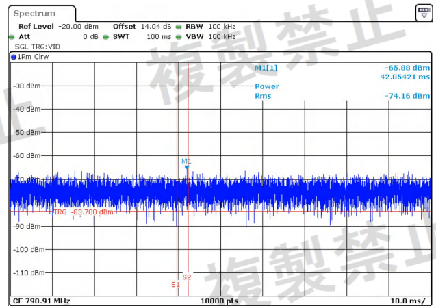
NTNV-11AC40MIMO-Ant2-5230-30~1000-PASS
