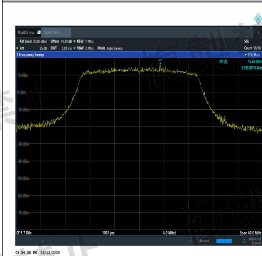
NTVN-11AX20MIMO-Ant3-5700-TPC_H-PASS
