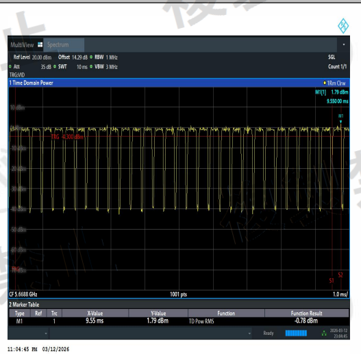
NTVN-11AX40MIMO-Ant3-5670-TPC_H-PASS
