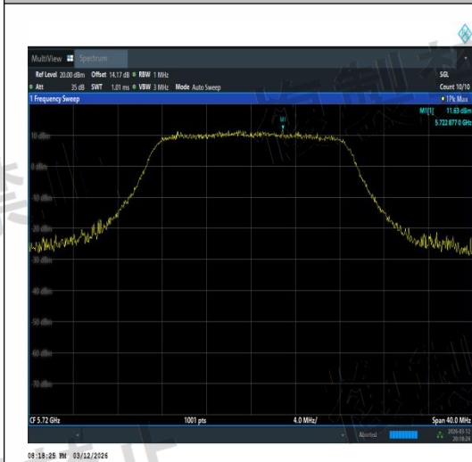
NTVN-11AC20MIMO-Ant3-5720-TPC_H-PASS
