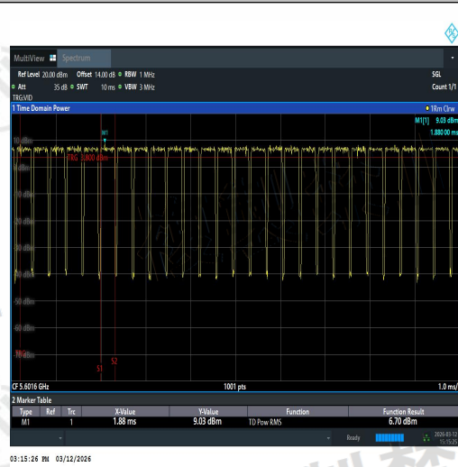
NTNV-11AX20SISO-Ant1-5600-TPC_H-PASS
