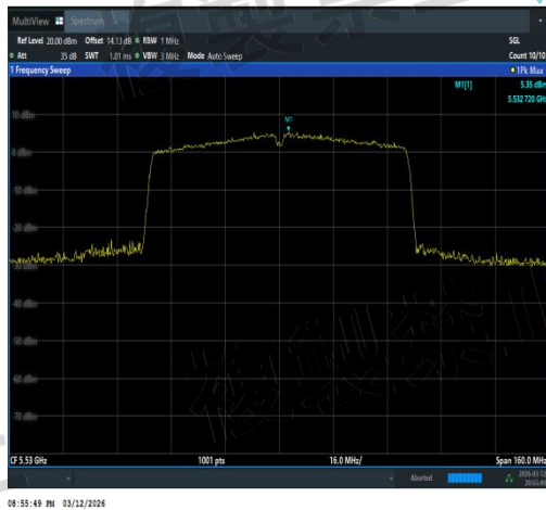
NTVN-11AC80MIMO-Ant2-5530-TPC_H-PASS
