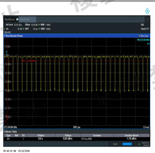
NTVN-11AC40MIMO-Ant3-5670-TPC_H-PASS
