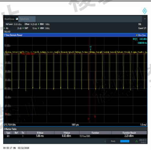
NTVN-11AX20MIMO-Ant3-5700-TPC_H-PASS
