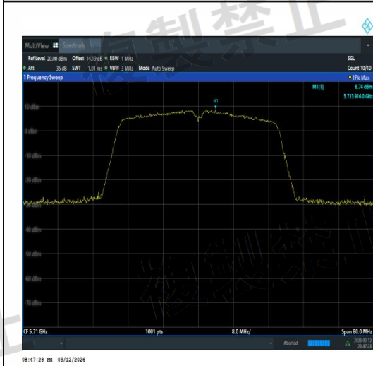
NTVN-11AC40MIMO-Ant1-5710-TPC_H-PASS
