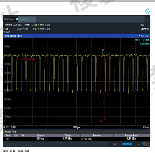
NTVN-11AC40MIMO-Ant3-5510-TPC_H-PASS
