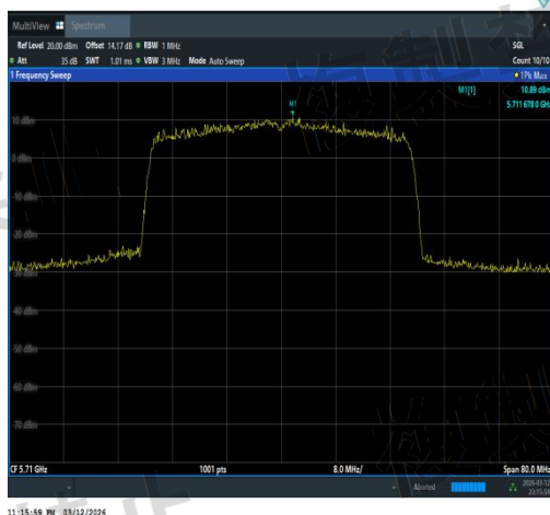
NTVN-11AX40MIMO-Ant3-5710-TPC_H-PASS
