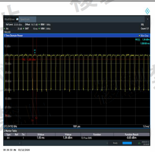
NTVN-11AC40MIMO-Ant3-5550-TPC_H-PASS
