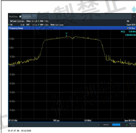
NTNV-11AC40SISO-Ant1-5510-TPC_H-PASS
