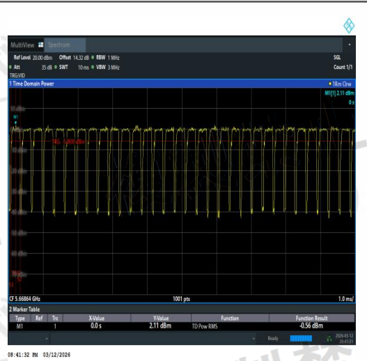
NTVN-11AC40MIMO-Ant1-5670-TPC_H-PASS
