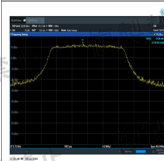
NTVN-11AX20MIMO-Ant3-5720-TPC_H-PASS
