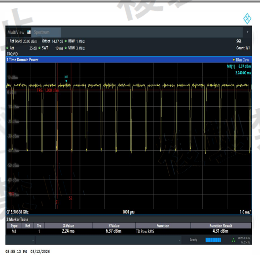
NTNV-11AX40SISO-Ant3-5510-TPC_H-PASS
