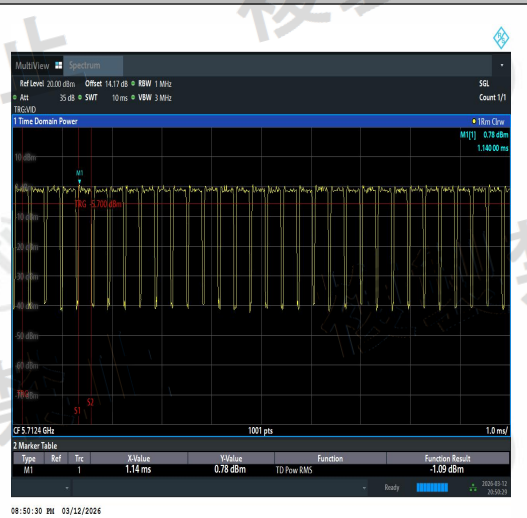
NTVN-11AC40MIMO-Ant3-5710-TPC_H-PASS
