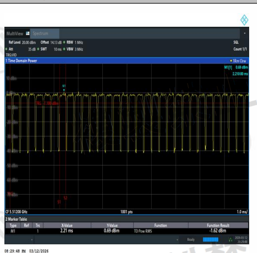
NTVN-11AC40MIMO-Ant1-5510-TPC_H-PASS
