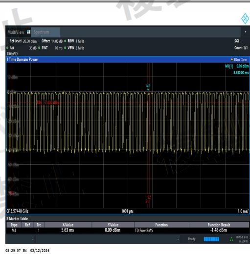
NTVN-11AC160SISO-Ant3-5570-TPC_H-PASS
