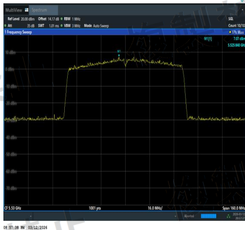
NTVN-11AC80MIMO-Ant3-5530-TPC_H-PASS
