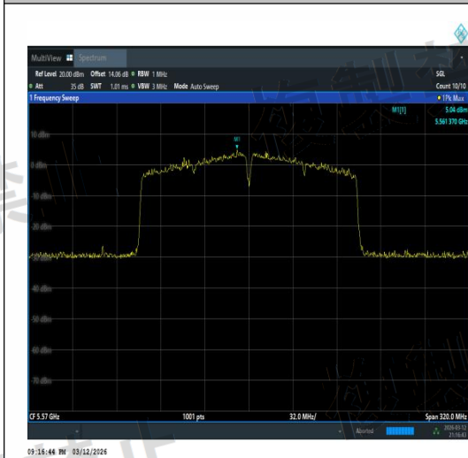
NTV-11AC160MIMO-Ant3-5570-TPC_H-PASS
