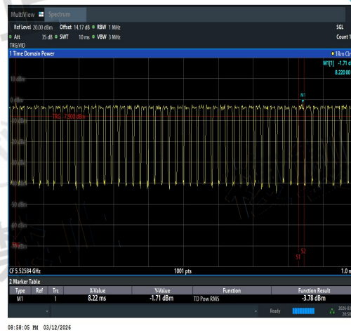
NTVN-11AC80MIMO-Ant3-5530-TPC_H-PASS
