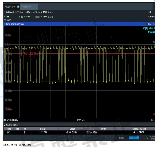
NTVN-11AC80MIMO-Ant1-5530-TPC_H-PASS
