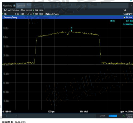
NTVN-11AC80MIMO-Ant2-5610-TPC_H-PASS
