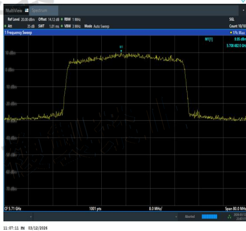
NTVN-11AX40MIMO-Ant1-5710-TPC_H-PASS
