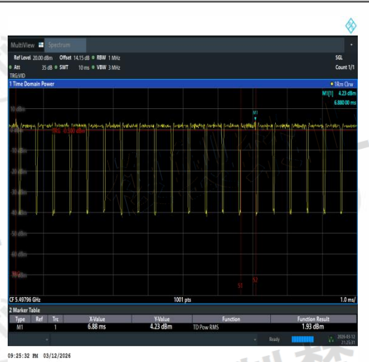
NTVN-11AX20MIMO-Ant1-5500-TPC_H-PASS
