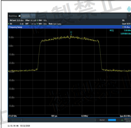
NTVN-11AX40MIMO-Ant1-5670-TPC_H-PASS
