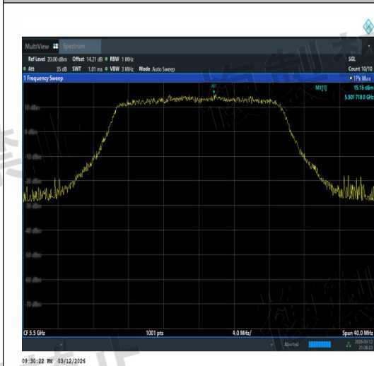
NTVN-11AX20MIMO-Ant3-5500-TPC_H-PASS
