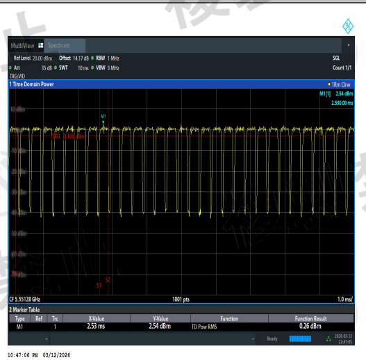
NTVN-11AX40MIMO-Ant3-5550-TPC_H-PASS
