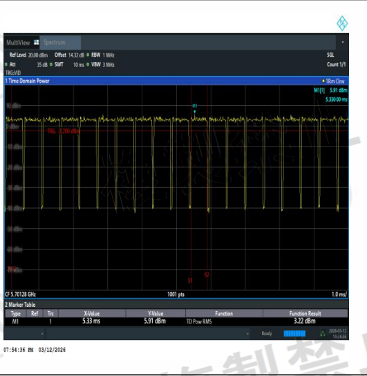
NTVN-11AC20MIMO-Ant2-5700-TPC_H-PASS
