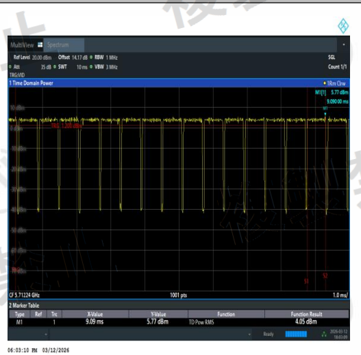
NTNV-11AX40SISO-Ant3-5710-TPC_H-PASS
