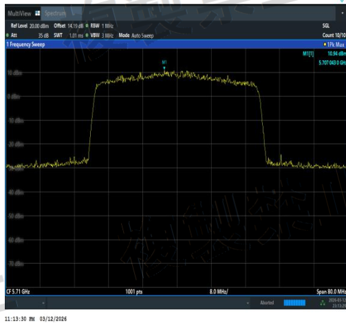
NTVN-11AX40MIMO-Ant2-5710-TPC_H-PASS
