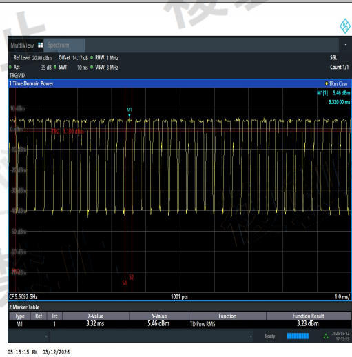
NTNV-11AC40SISO-Ant3-5510-TPC_H-PASS
