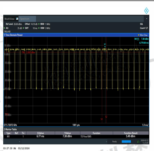
NTNV-11AX20SISO-Ant1-5720-TPC_H-PASS
