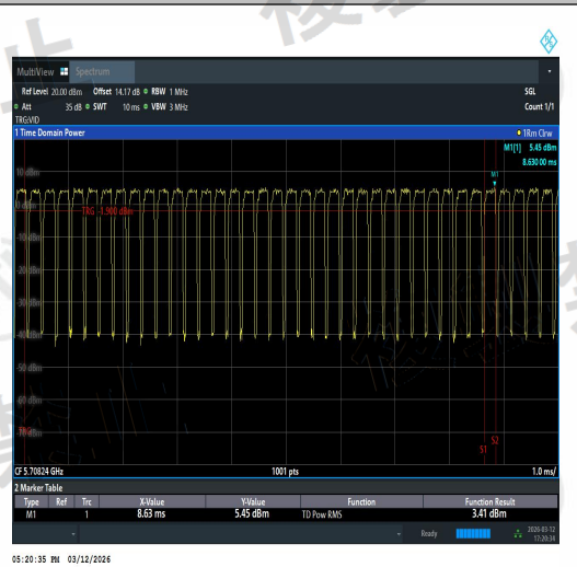
NTNV-11AC40SISO-Ant3-5710-TPC_H-PASS
