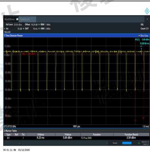
NTNV-11AX40SISO-Ant3-5670-TPC_H-PASS
