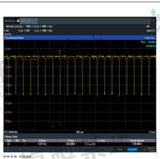
NTVN-11AX20MIMO-Ant1-5700-TPC_H-PASS
