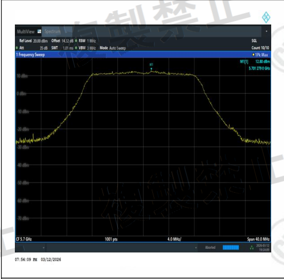
NTVN-11AC20MIMO-Ant2-5700-TPC_H-PASS
