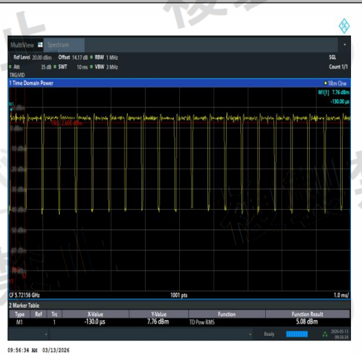
NTNV-11AX20SISO-Ant3-5720-TPC_H-PASS
