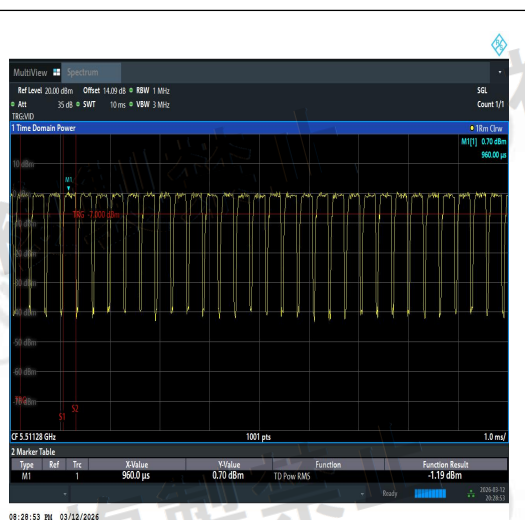
NTVN-11AC40MIMO-Ant1-5510-TPC_H-PASS
