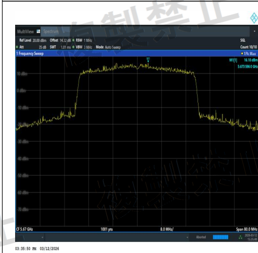
NTNV-11AX40SISO-Ant1-5670-TPC_H-PASS
