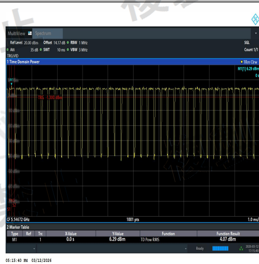
NTNV-11AC40SISO-Ant3-5550-TPC_H-PASS
