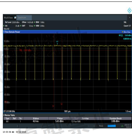
NTNV-11AC40SISO-Ant1-5510-TPC_H-PASS
