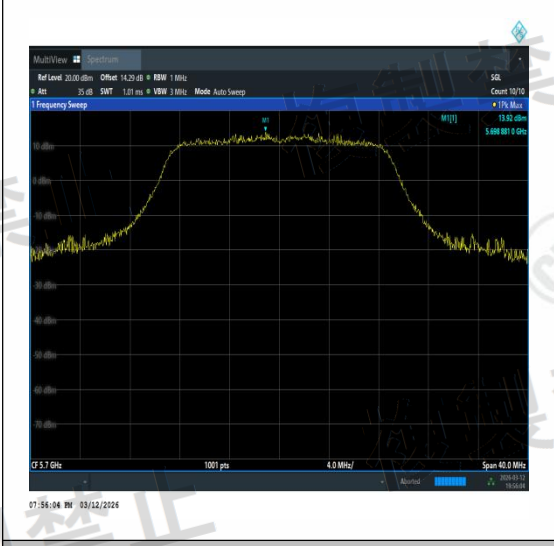
NTVN-11AC20MIMO-Ant3-5700-TPC_H-PASS
