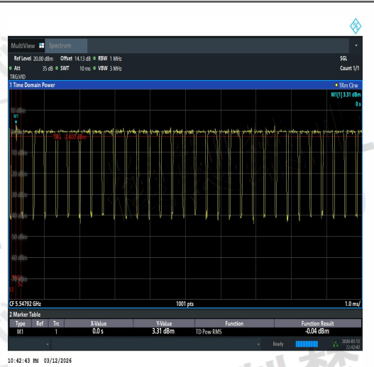
NTVN-11AX40MIMO-Ant1-5550-TPC_H-PASS
