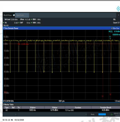
NTNV-11AC40SISO-Ant1-5550-TPC_H-PASS
