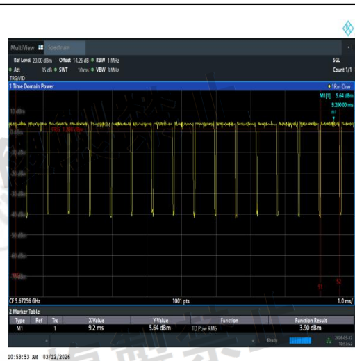
NTNV-11AX40SISO-Ant1-5670-TPC_H-PASS
