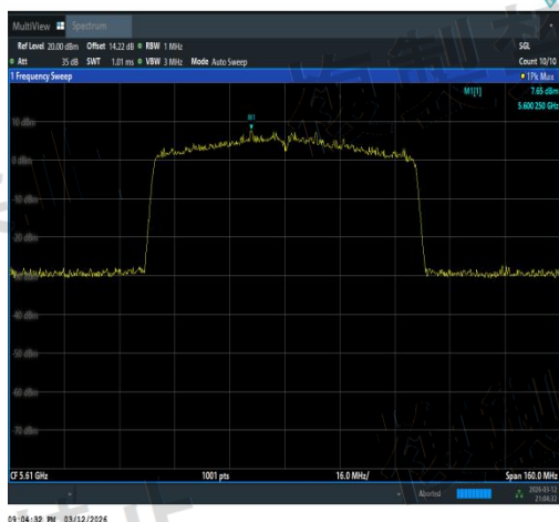
NTVN-11AC80MIMO-Ant3-5610-TPC_H-PASS
