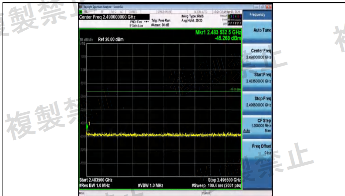
NTLV-3DH5-Ant1-2480-2483.5~2496.5-PASS
