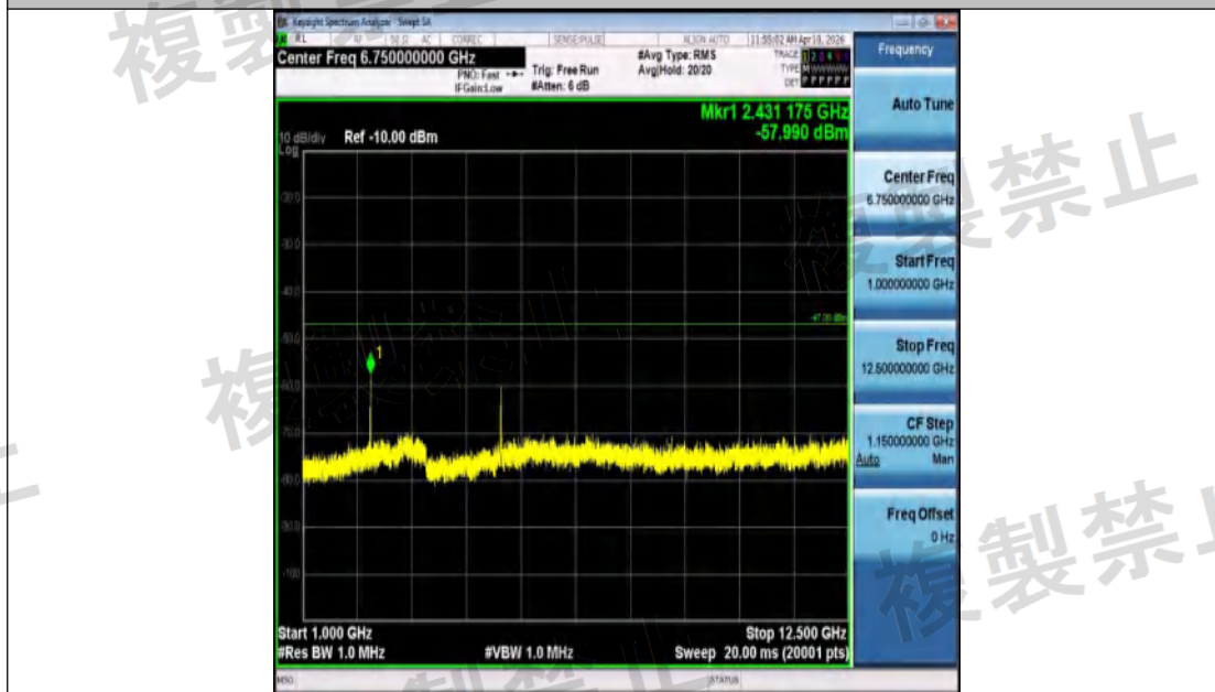
NTHV-DH5-Ant1-2402-1000~12500-PASS
