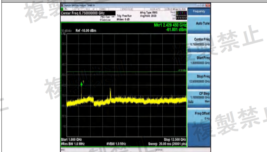
NTLV-DH5-Ant1-2441-1000~12500-PASS
