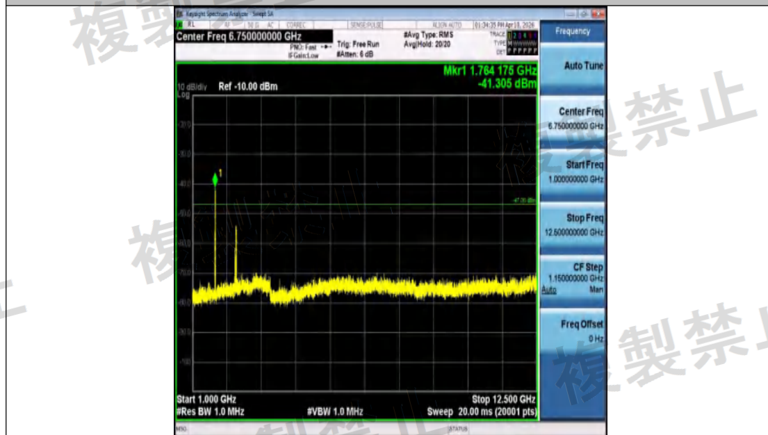
NTLV-3DH5-Ant1-2402-1000~12500-See table below
