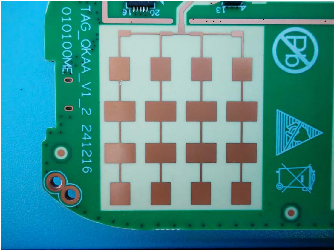
Radar Antenna (TX)
