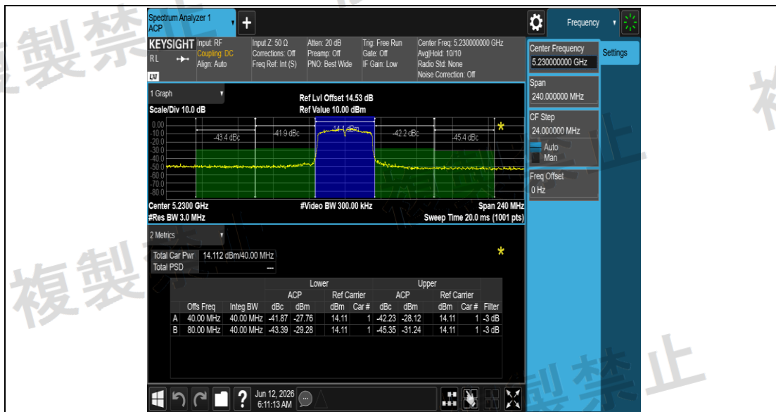
NTNV_11N40SISO_Ant1_5230
