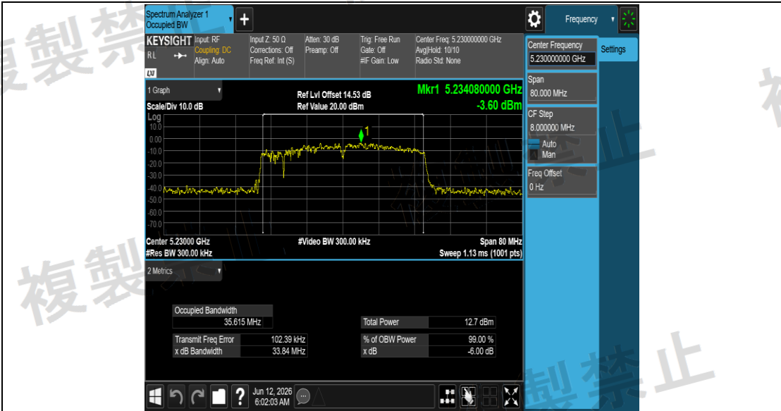
NTNV_11N40SISO_Ant1_5230
