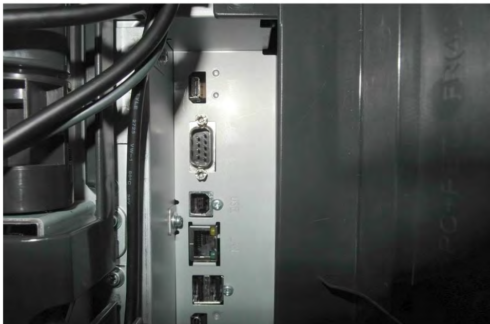
EUT Photo (32)
