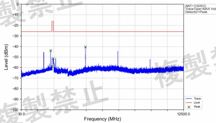
Pi/4DQPSK_2DH5_2480MHz_Ant1_NTLV
