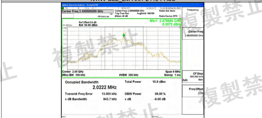
NTNV-BLE 2M-Ant1-2480-PASS
