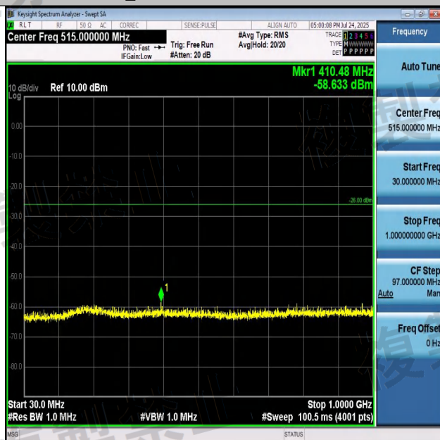
NTNV-BLE_1M-Ant1-2480-30~1000-PASS
