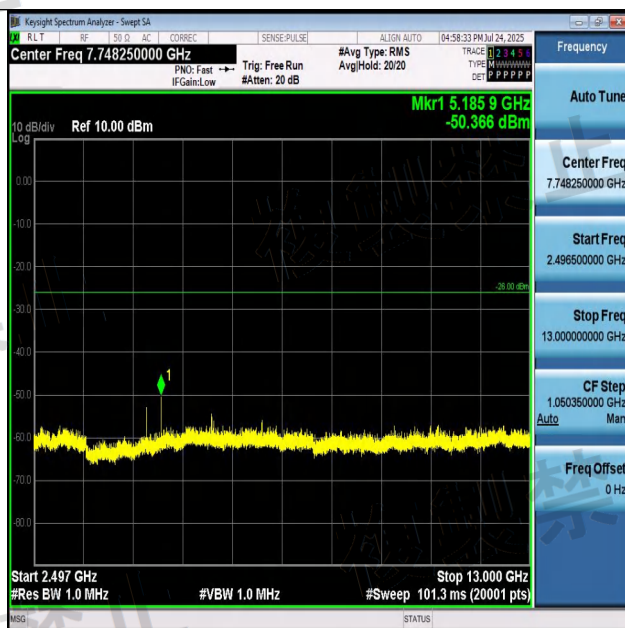
NTNV-BLE_1M-Ant1-2440-2496.5~13000-PASS
