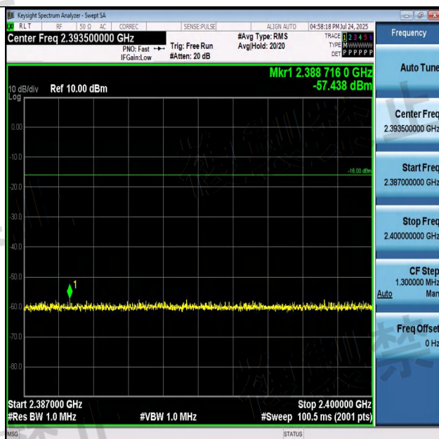
NTNV-BLE_1M-Ant1-2440-2387~2400-PASS
