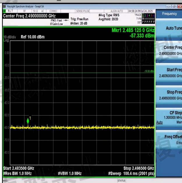
NTNV-BLE_1M-Ant1-2440-2483.5~2496.5-PASS
