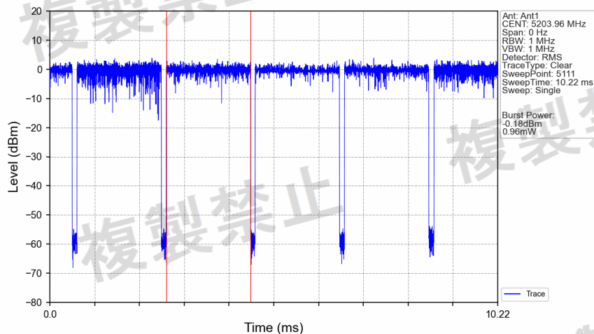
802.11ac(VHT20)_MCH_5200MHz_Ant1_NTNV
