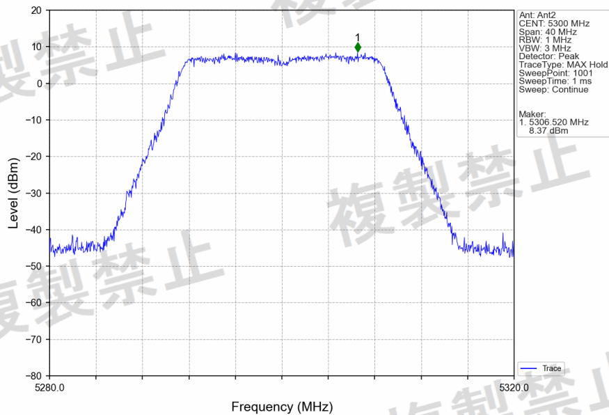
802.11ac(VHT20)_MCH_5300MHz_Ant2_NTNV
