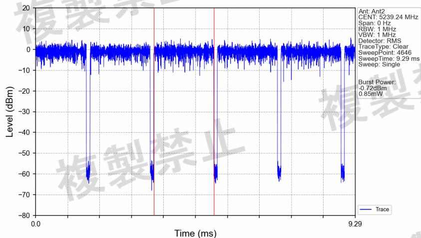
802.11ax(HEW20)_HCH_5240MHz_RU242_Left_Ant2_NTNV
