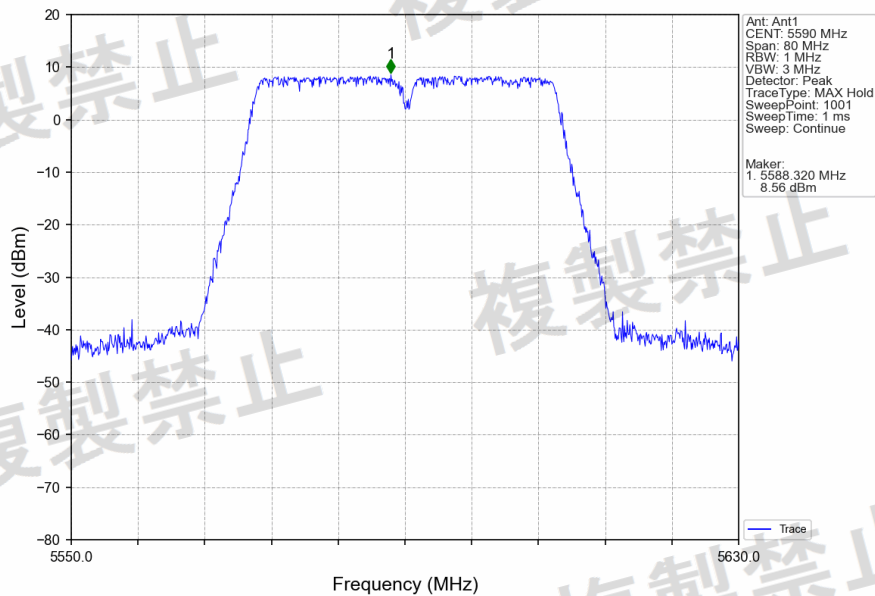
802.11ac(VHT40)_MCH_5590MHz_Ant1_NTNV
