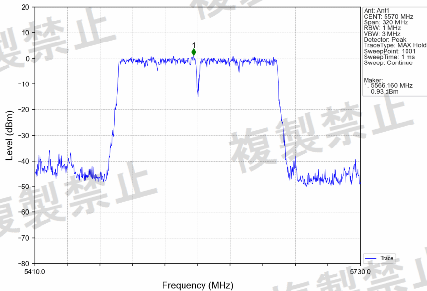
802.11ac(VHT160)_MCH_5570MHz_Ant1_NTNV
