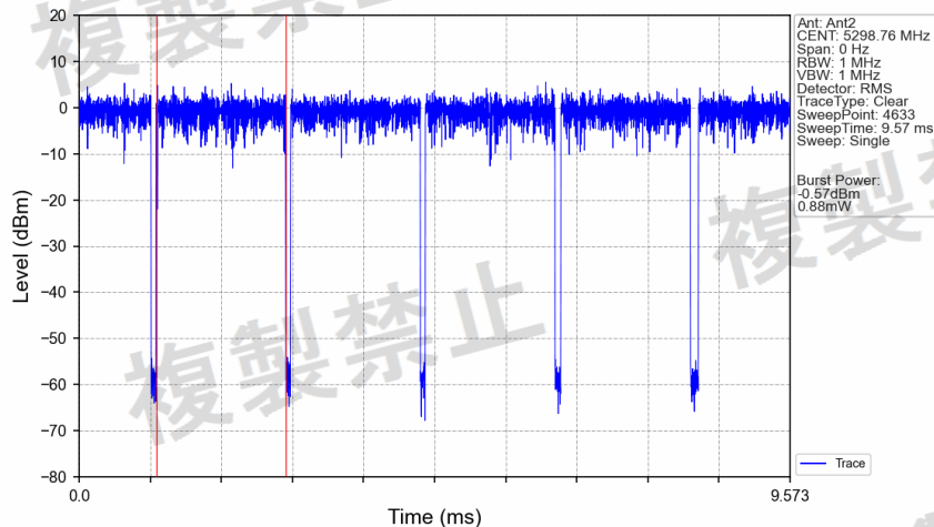
802.11ax(HEW20)_MCH_5300MHz_RU242_Left_Ant2_NTNV
