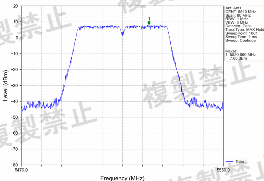
802.11ac(VHT40)_LCH_5510MHz_Ant1_NTNV
