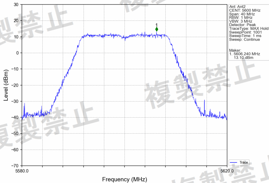
802.11ac(VHT20)_MCH_5600MHz_Ant2_NTNV
