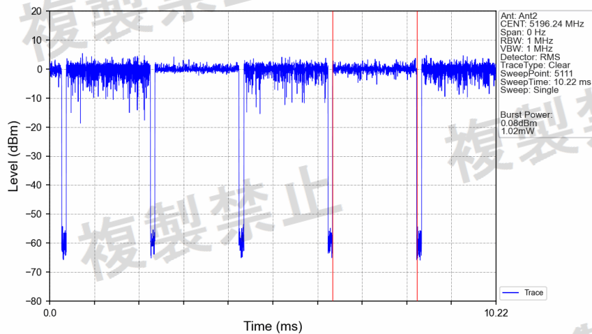
802.11ac(VHT20)_MCH_5200MHz_Ant2_NTNV
