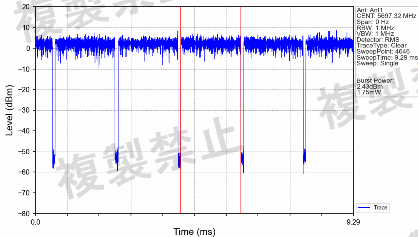
802.11ax(HEW20)_HCH_5700MHz_RU242_Left_Ant1_NTNV
