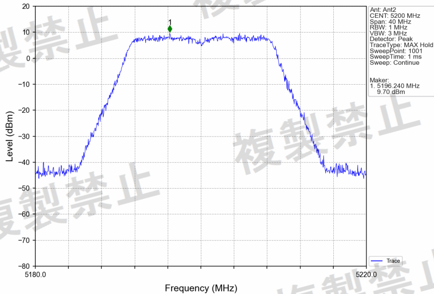
802.11ac(VHT20)_MCH_5200MHz_Ant2_NTNV
