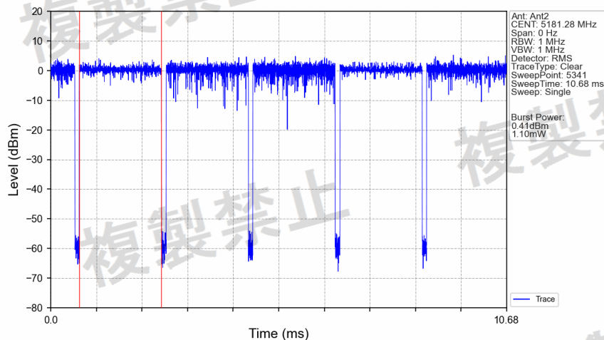
802.11ac(VHT20)_LCH_5180MHz_Ant2_NTNV
