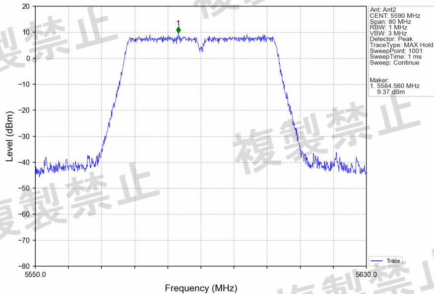
802.11ac(VHT40)_MCH_5590MHz_Ant2_NTNV
