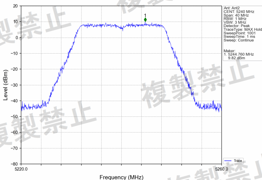
802.11ac(VHT20)_HCH_5240MHz_Ant2_NTNV
