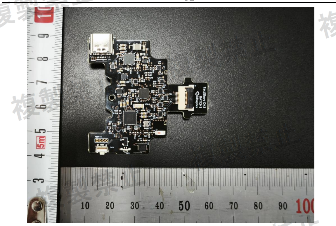
Main Board Top_EUT
