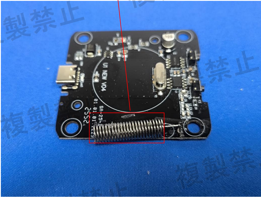
315MHz RX Ant.
