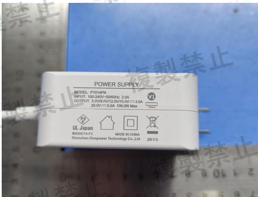
Photo 7 Adapter Appearance
