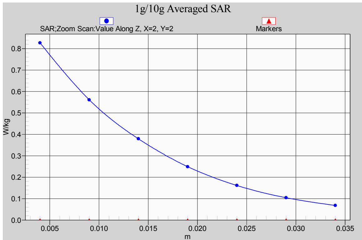
Fig. 26-1 Z-Scan at power reference point (1900 MHz CH512)
