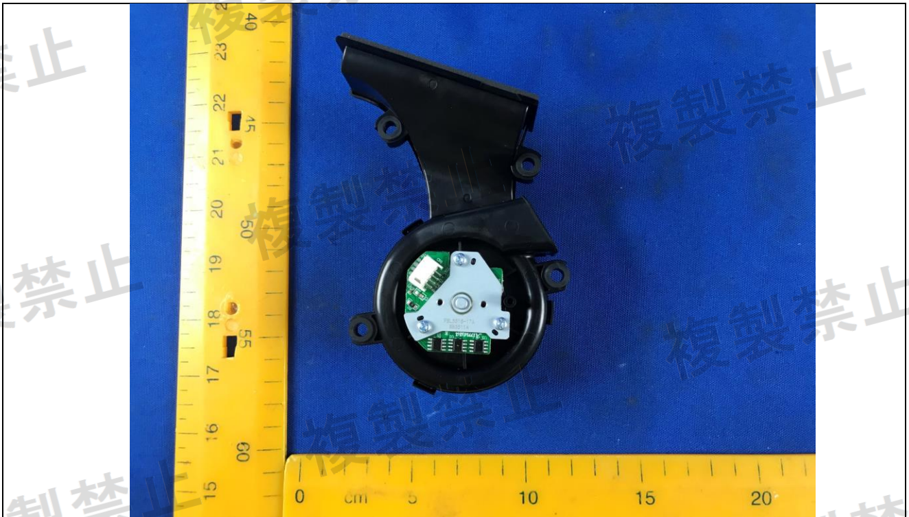
Details of: Suction motor
