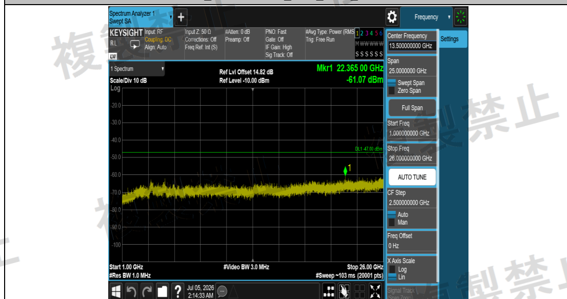
NTNV_11AC40SISO_Ant1_5510_1000~26000
