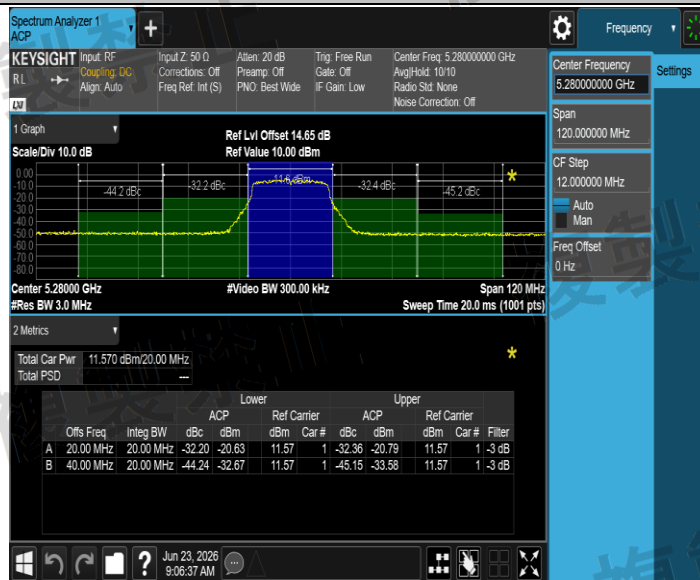
NTNV_11N20SISO_Ant1_5280
