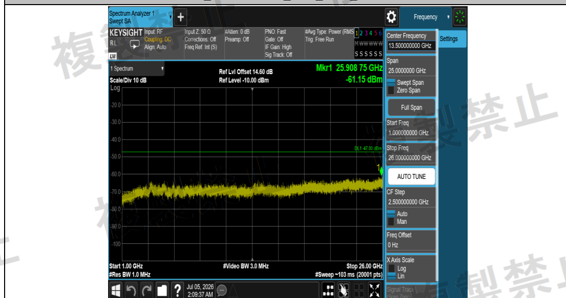
NTNV_11AC20SISO_Ant1_5720_1000~26000
