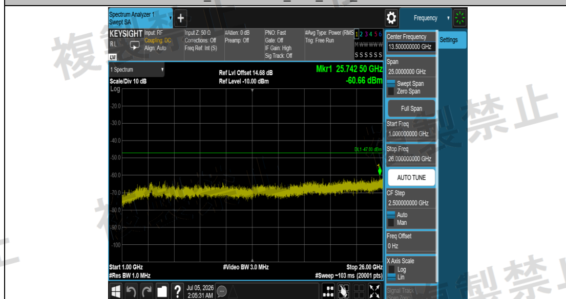
NTNV_11AC20SISO_Ant1_5260_1000~26000
