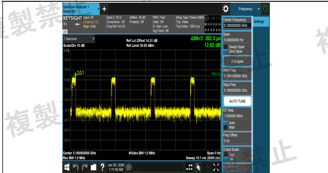
NTNV_11AX20SISO_Ant1_5180
