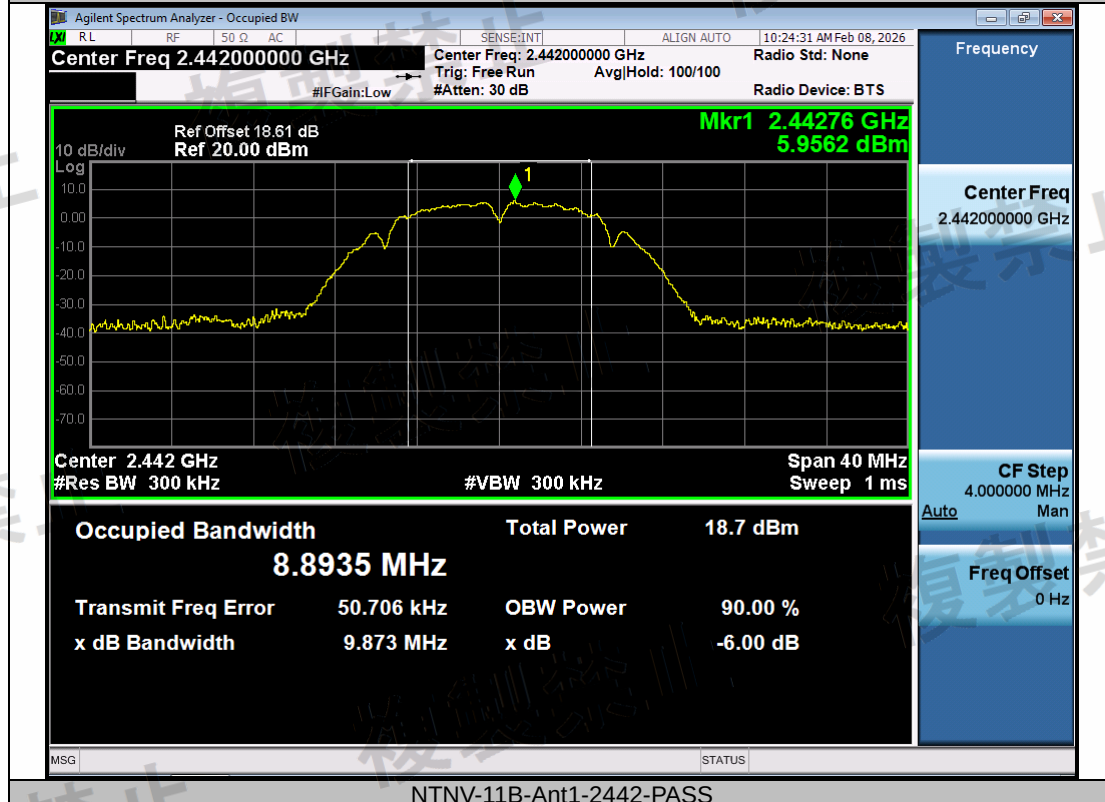
NTNV-11B-Ant1-2442-PASS
