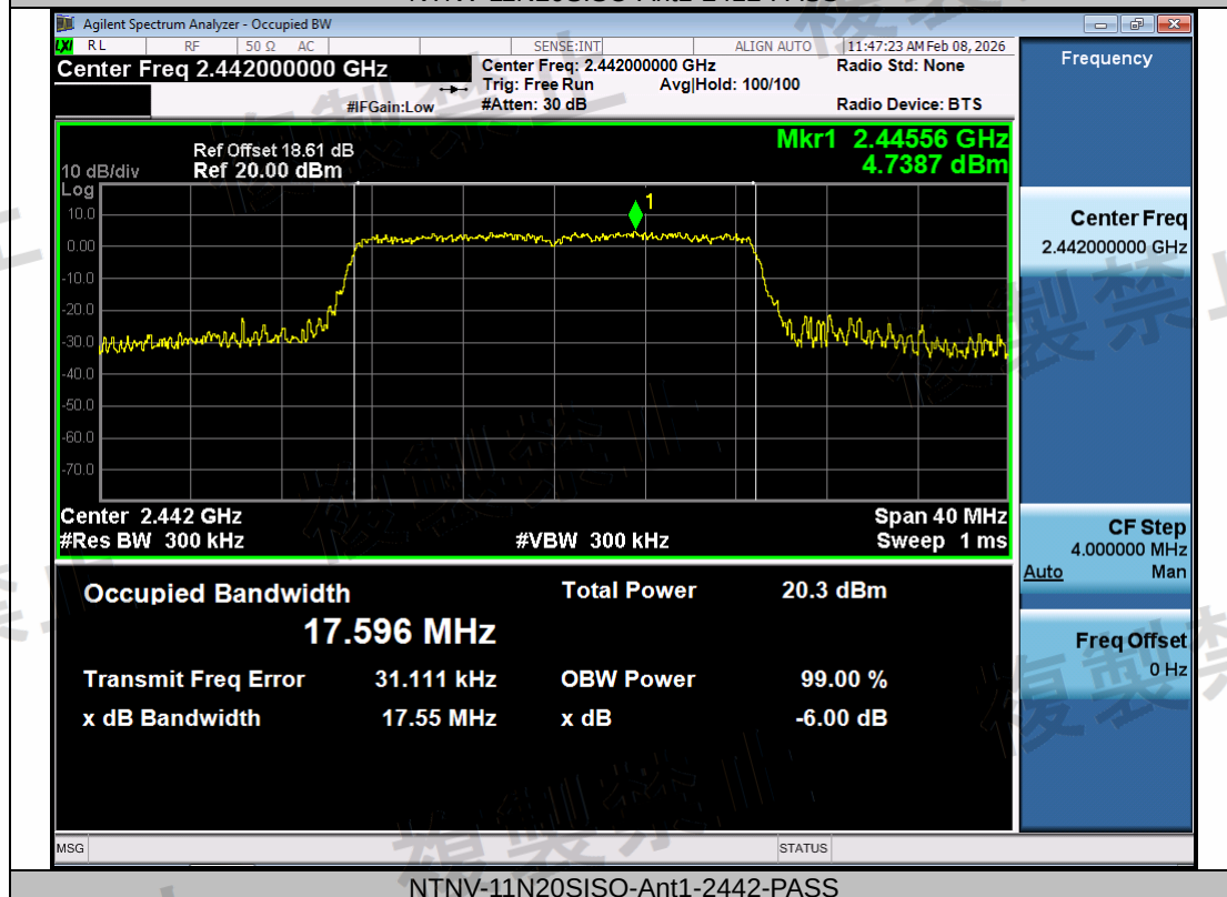
NTNV-11N20SISO-Ant1-2442-PASS
