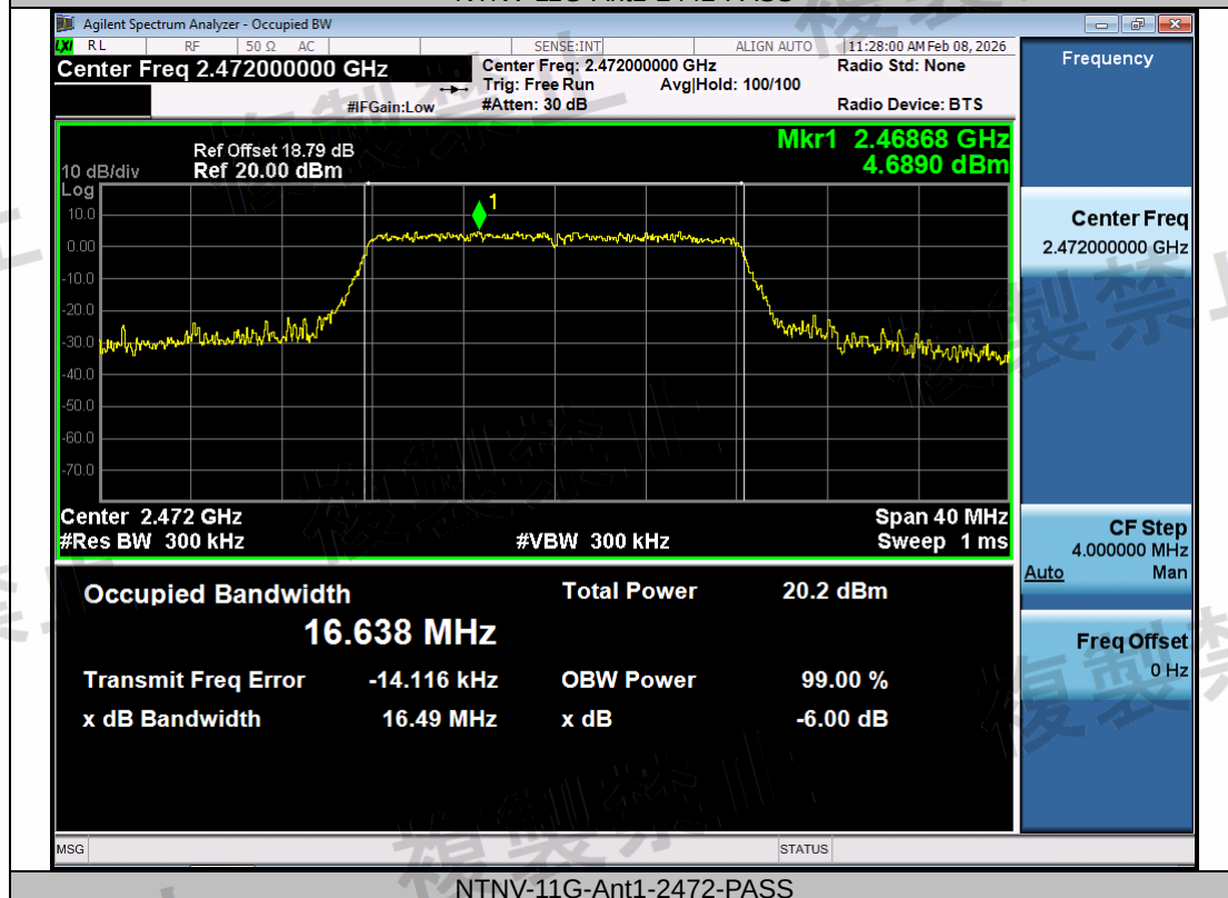
NTNV-11G-Ant1-2472-PASS
