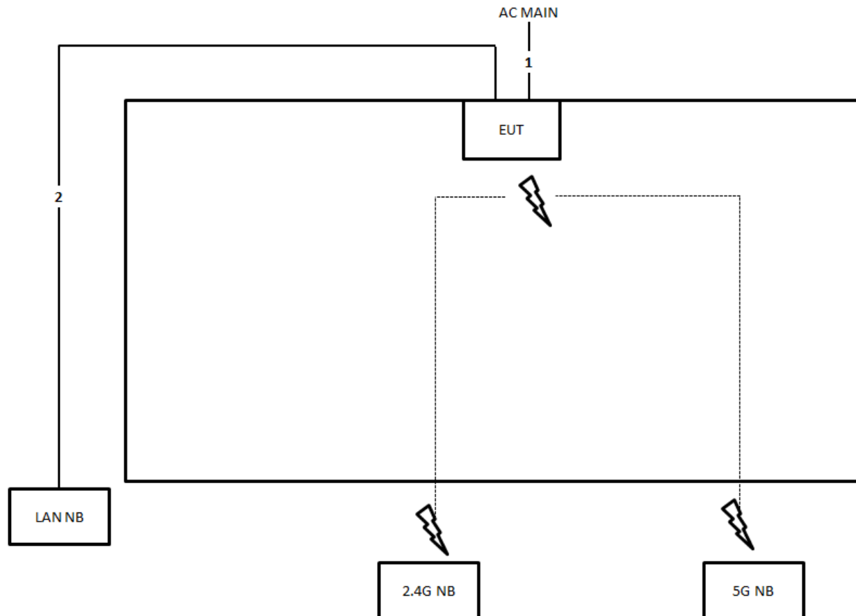
Test Setup Diagram - Radiated Test < 1GHz / Unintentional - Normal Link
