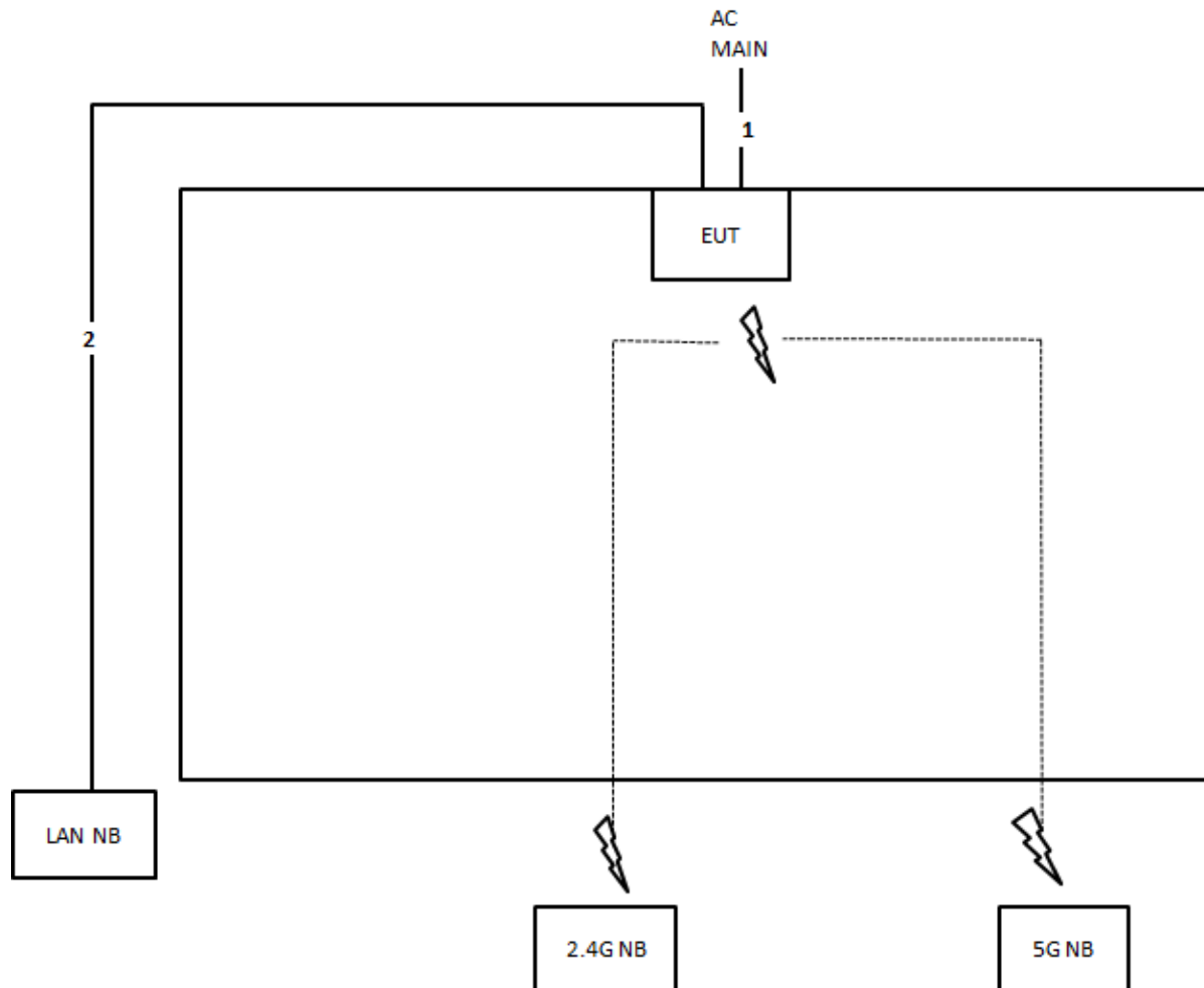
Test Setup Diagram - Radiated Test > 1GHz / Unintentional 1GHz~5 th - Normal Link
