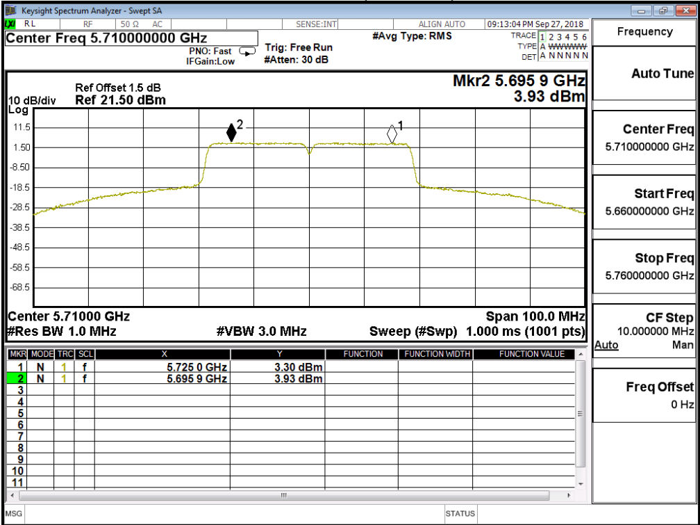
Channel 142(U-NII-2C)
