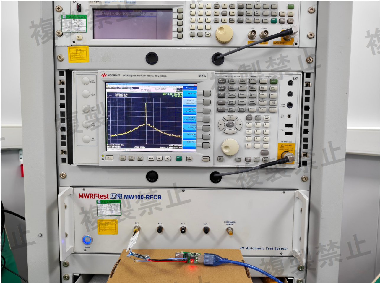
RF Conducted Test View-left
