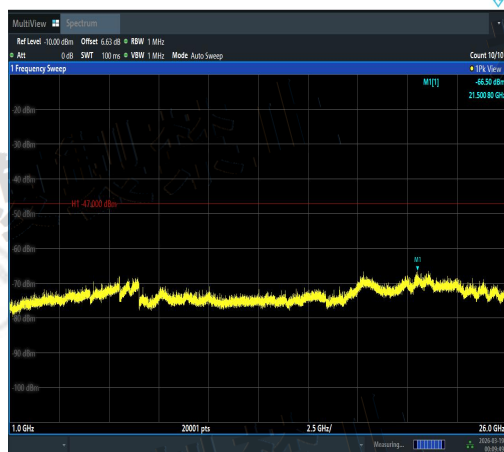
NTNV-11N40MIMO-Ant3-5710-1000~26000-PAS
