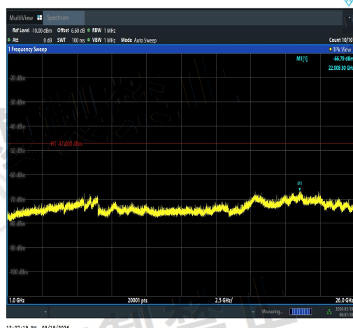
NTNV-11N40MIMO-Ant3-5550-1000~26000-PAS
