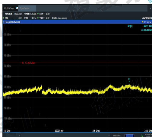
NTNV-11AC20SISO-Ant1-5500-1000~26000-PA
