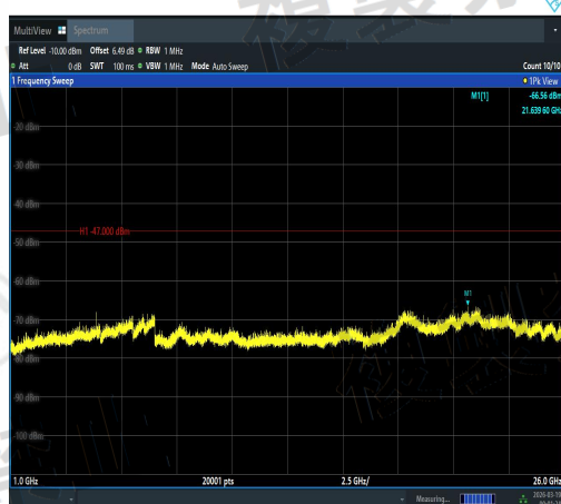
NTNV-11N20MIMO-Ant1-5600-1000~26000-PAS
