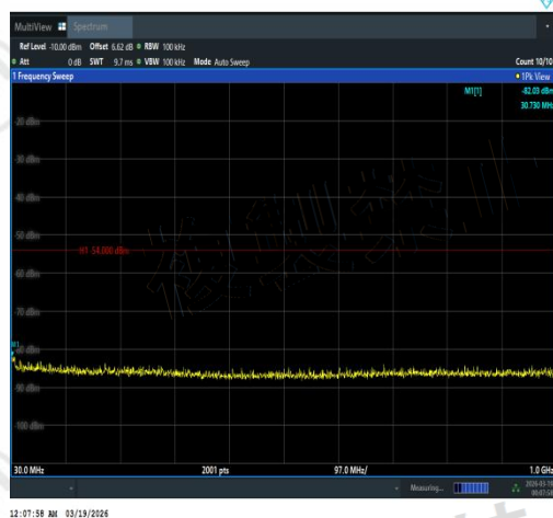
NTNV-11N40MIMO-Ant2-5670-30~1000-PASS
