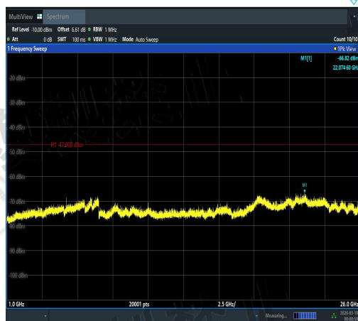
NTNV-11N20MIMO-Ant3-5500-1000~26000-PAS
