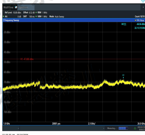
NTNV-11N40MIMO-Ant2-5550-1000~26000-PAS
