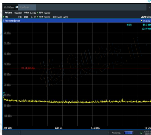
NTNV-11N20MIMO-Ant2-5600-30~1000-PASS
