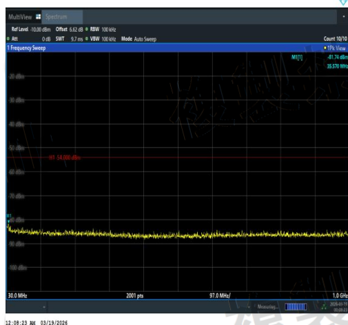
NTNV-11N40MIMO-Ant3-5670-30~1000-PASS
