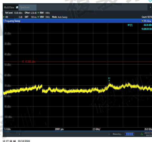
NTNV-11N40MIMO-Ant1-5670-1000~26000-PAS
