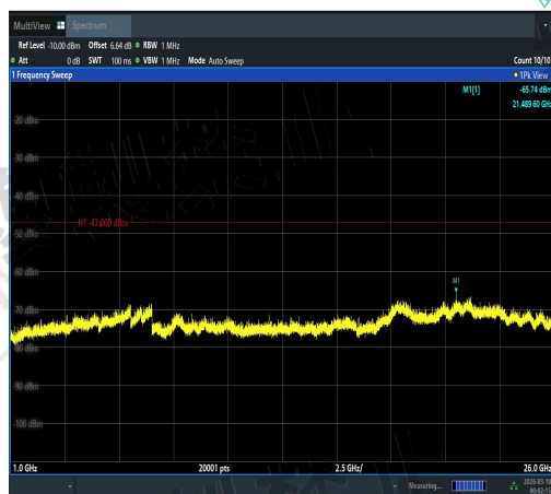
NTNV-11N20MIMO-Ant3-5600-1000~26000-PAS
