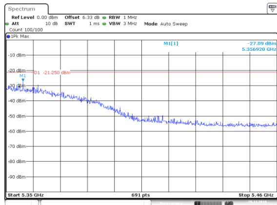
VHT80, M0.1 to M9.1 5290 MHz Peak
