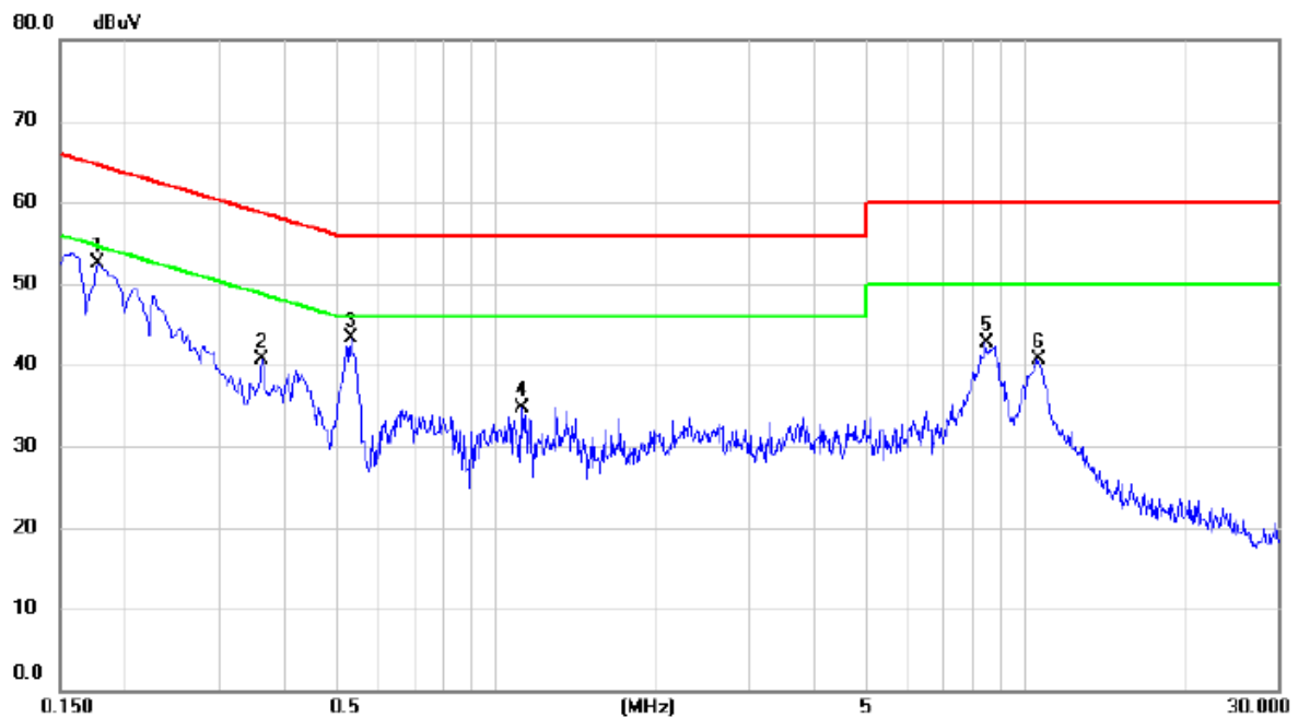
Phase: Line
