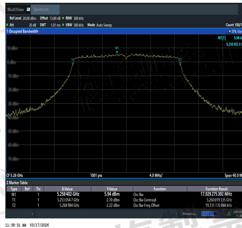
NTNV-11AC20SISO-Ant2-5260-PASS
