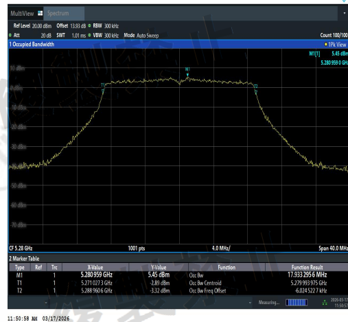
NTNV-11AC20SISO-Ant3-5280-PASS
