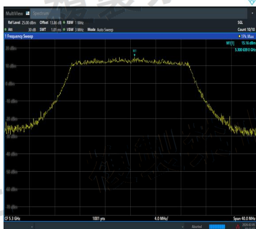
NTNV-11AX20SISO-Ant1-5300-TPC_H-PASS
