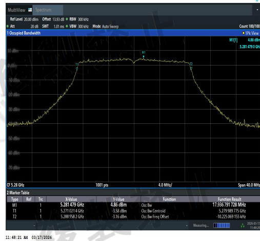
NTVN-11N20SISO-Ant3-5280-PASS
