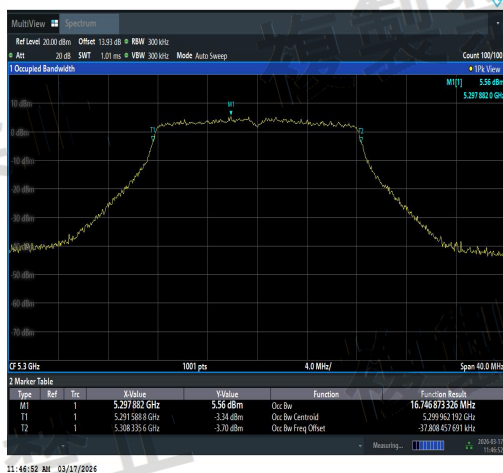
NTNV-11A-Ant3-5300-PASS
