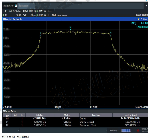
NTNV-11AX20SISO-Ant1-5300-PASS
