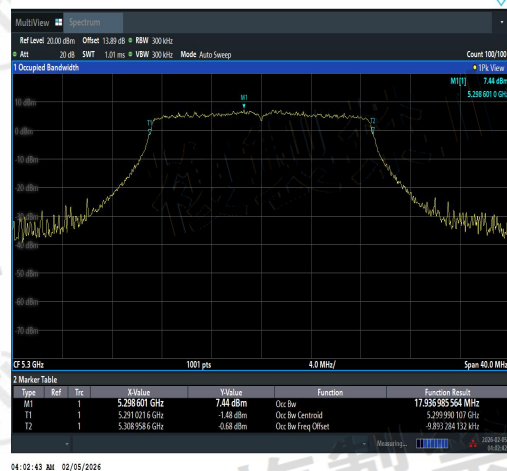
NTVN-11N20SISO-Ant2-5300-PASS
