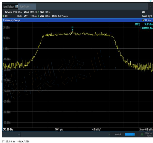
NTNV-11AX20SISO-Ant3-5320-TPC_H-PASS
