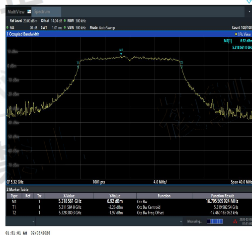
NTNV-11A-Ant1-5320-PASS
