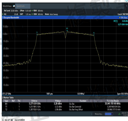
NTNV-11AC40SISO-Ant3-5270-PASS
