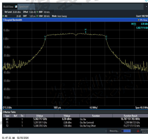
NTNV-11A-Ant1-5300-PASS
