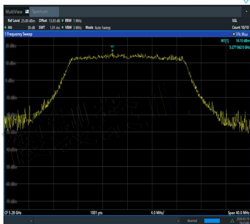
NTNV-11AX20SISO-Ant3-5280-TPC_H-PASS
