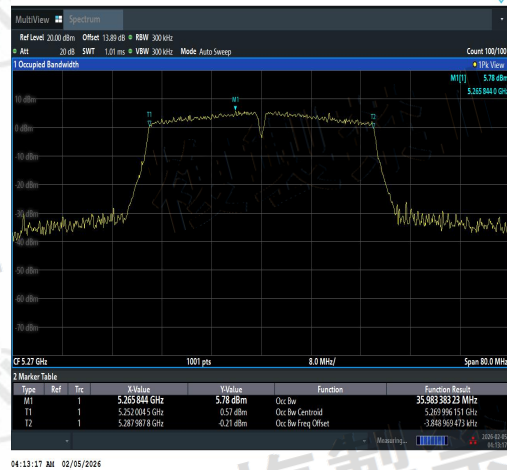
NTNV-11N40SISO-Ant2-5270-PASS
