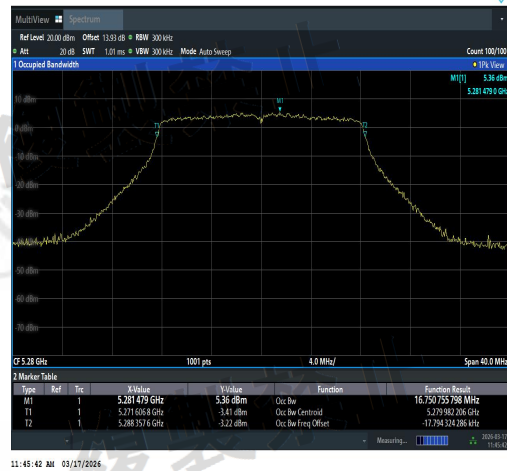
NTNV-11A-Ant3-5280-PASS
