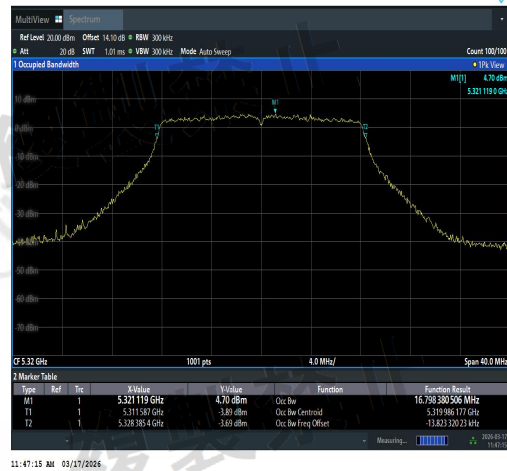
NTNV-11A-Ant3-5320-PASS
