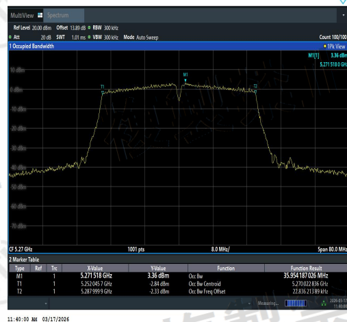
NTNV-11AC40SISO-Ant2-5270-PASS
