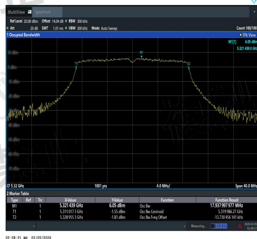
NTVN-11N20SISO-Ant1-5320-PASS
