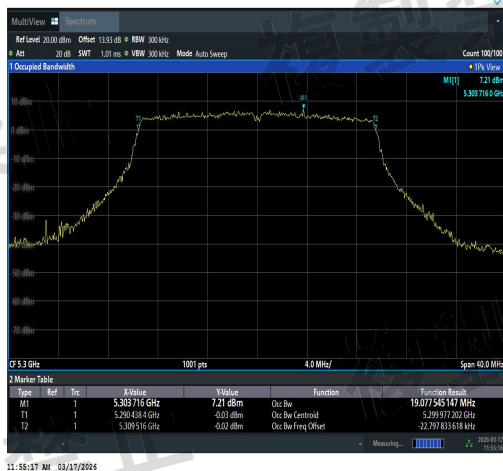
NTNV-11AX20SISO-Ant3-5300-PASS
