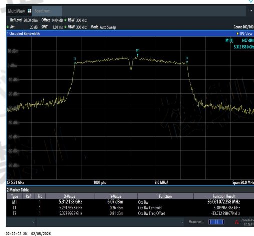
NTNV-11N40SISO-Ant1-5310-PASS
