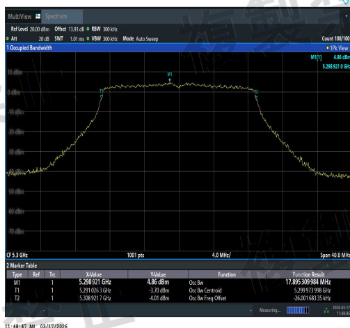
NTVN-11N20SISO-Ant3-5300-PASS
