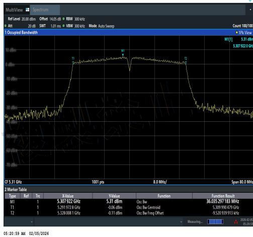
NTNV-11N40SISO-Ant2-5310-PASS
