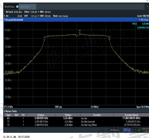
NTNV-11AC20SISO-Ant2-5300-PASS
