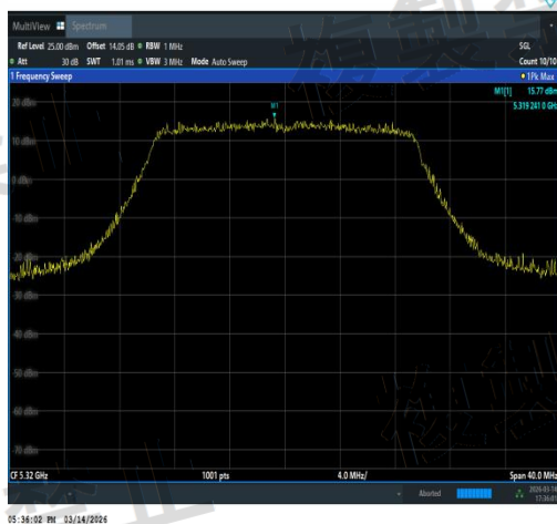
NTNV-11AX20SISO-Ant2-5320-TPC_H-PASS
