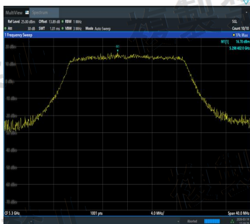
NTNV-11AX20SISO-Ant2-5300-TPC_H-PASS
