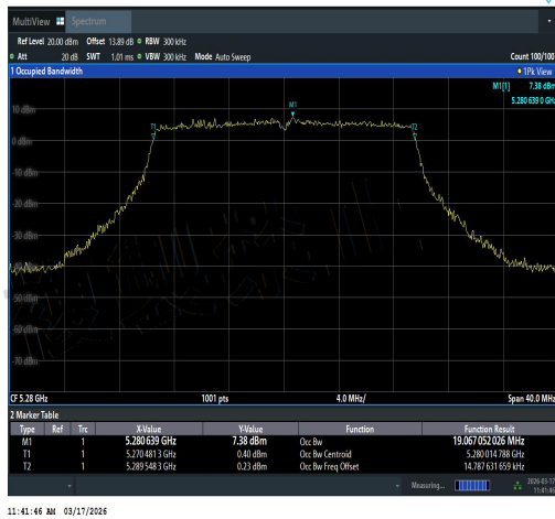
NTNV-11AX20SISO-Ant2-5280-PASS
