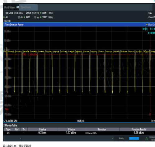
NTNV-11AX20MIMO-Ant2-5260-TPC_H-PASS
