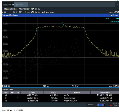
NTNV-11A-Ant2-5280-PASS
