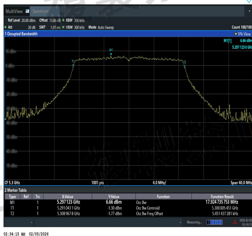
NTNV-11AC20SISO-Ant1-5300-PASS
