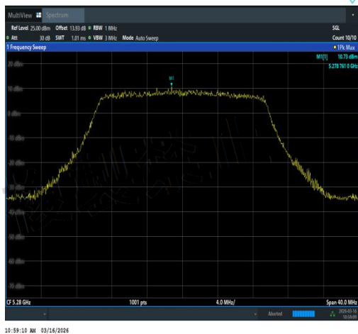
NTVN-11AX20MIMO-Ant3-5280-TPC_H-PASS
