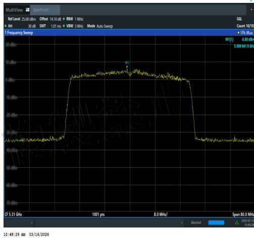
NTNV-11AX40MIMO-Ant3-5310-TPC_H-PASS
