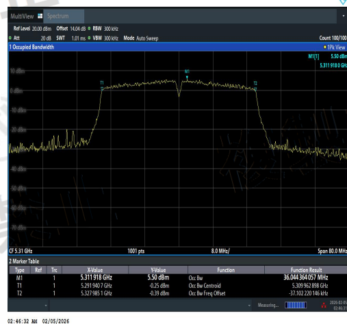
NTNV-11AC40SISO-Ant1-5310-PASS
