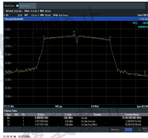
NTNV-11AC40SISO-Ant3-5310-PASS
