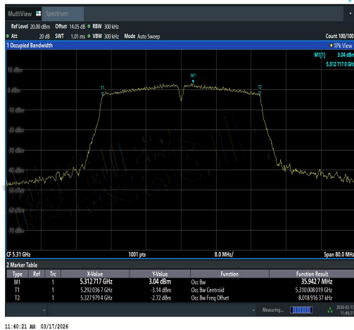
NTNV-11AC40SISO-Ant2-5310-PASS
