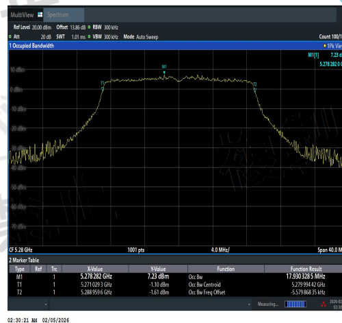
NTNV-11AC20SISO-Ant1-5280-PASS
