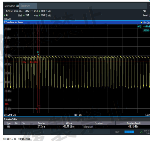
NTNV-11AC160MIMO-Ant3-5250-TPC_H-PASS
