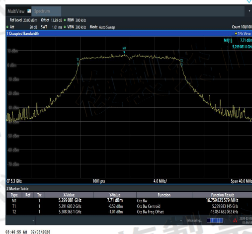
NTNV-11A-Ant2-5300-PASS
