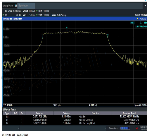
NTNV-11N20SISO-Ant2-5320-PASS
