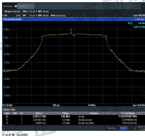
NTNV-11AC20SISO-Ant3-5260-PASS
