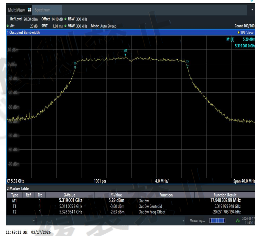
NTNV-11N20SISO-Ant3-5320-PASS
