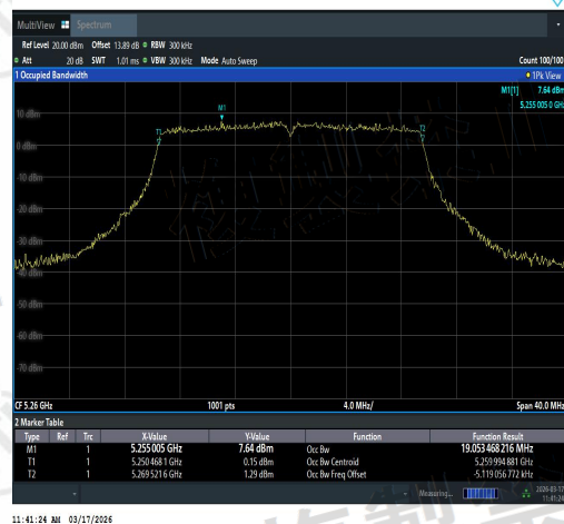
NTVN-11AX20SISO-Ant2-5260-PASS
