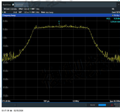
NTNV-11AX20SISO-Ant1-5280-TPC_H-PASS
