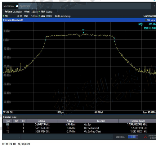
NTNV-11AC20SISO-Ant1-5260-PASS
