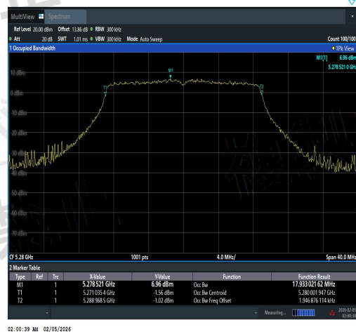
NTNV-11N20SISO-Ant1-5280-PASS
