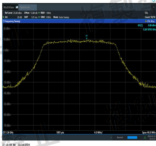
NTNV-11AX20MIMO-Ant2-5260-TPC_H-PASS
