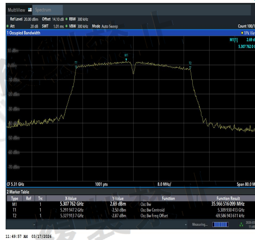
NTNV-11N40SISO-Ant3-5310-PASS
