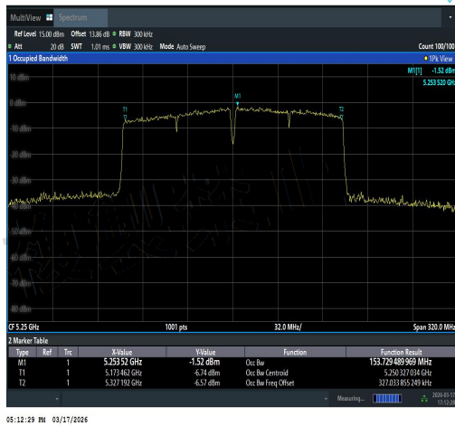
NTVN-11AC160SISO-Ant2-5250-PASS
