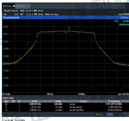
NTNV-11AC20SISO-Ant3-5300-PASS
