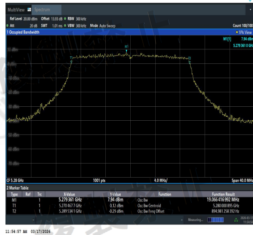
NTNV-11AX20SISO-Ant3-5280-PASS
