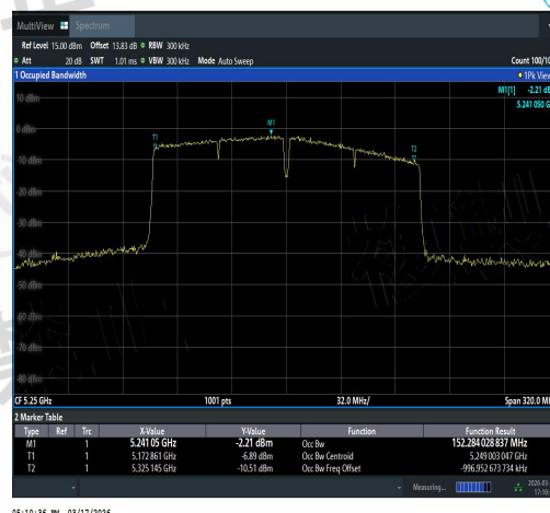
NTNV-11AC160SISO-Ant1-5250-PASS
