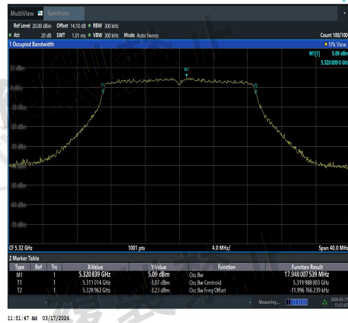
NTNV-11AC20SISO-Ant3-5320-PASS
