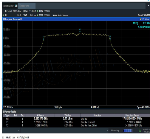
NTNV-11AC20SISO-Ant2-5280-PASS
