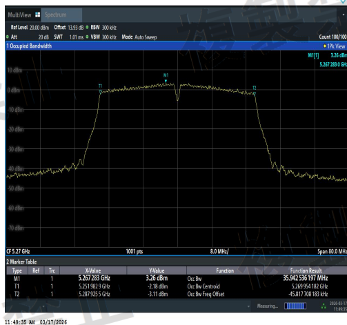
NTNV-11N40SISO-Ant3-5270-PASS
