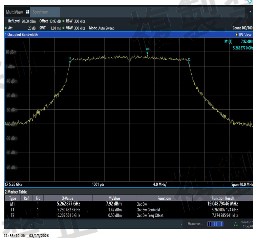
NTVN-11AX20SISO-Ant3-5260-PASS
