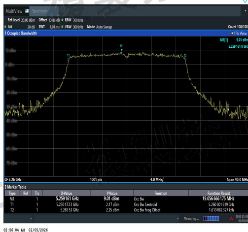
NTVN-11AX20SISO-Ant1-5260-PASS
