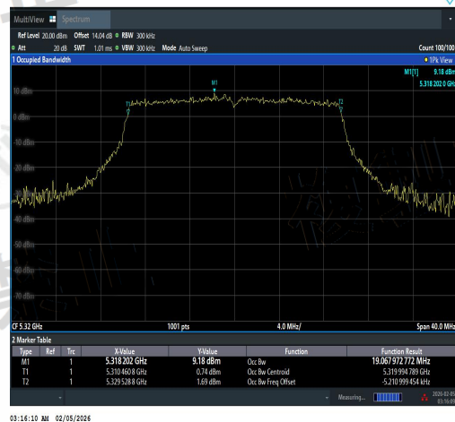
NTNV-11AX20SISO-Ant1-5320-PASS
