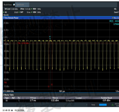
NTNV-11AX40MIMO-Ant3-5310-TPC_H-PASS
