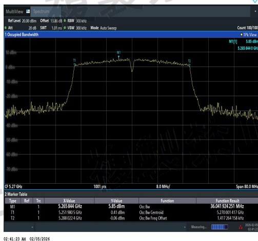
NTNV-11AC40SISO-Ant1-5270-PASS
