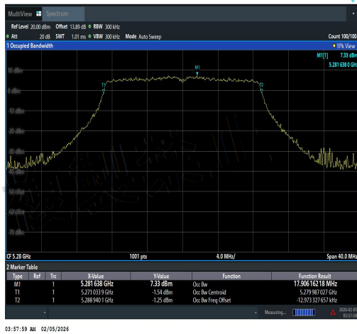
NTVN-11N20SISO-Ant2-5280-PASS
