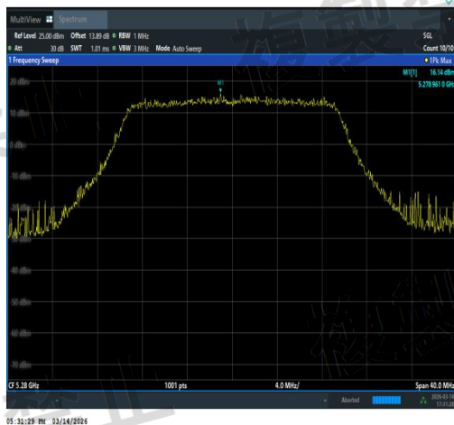
NTNV-11AX20SISO-Ant2-5280-TPC_H-PASS
