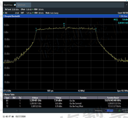
NTNV-11AX20SISO-Ant2-5300-PASS
