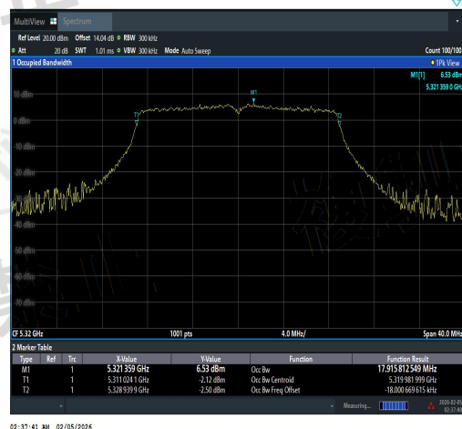
NTNV-11AC20SISO-Ant1-5320-PASS
