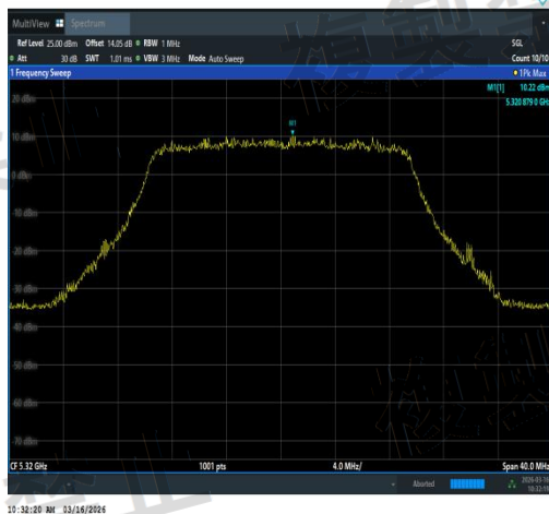
NTVN-11AX20MIMO-Ant2-5320-TPC_H-PASS
