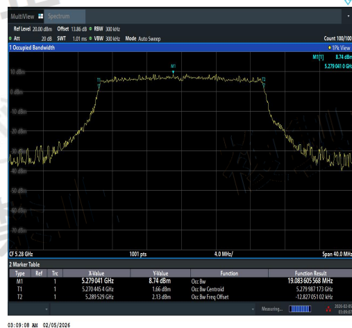
NTVN-11AX20SISO-Ant1-5280-PASS
