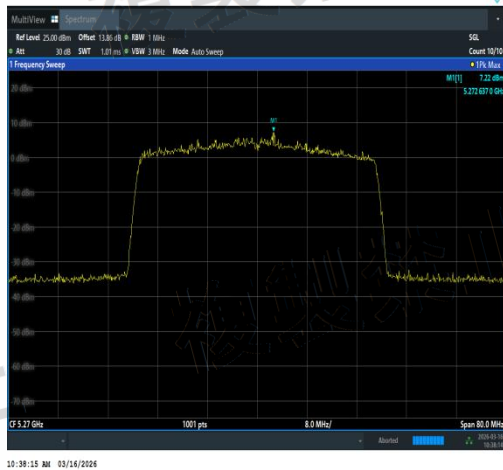
NTNV-11AX40MIMO-Ant1-5270-TPC_H-PASS
