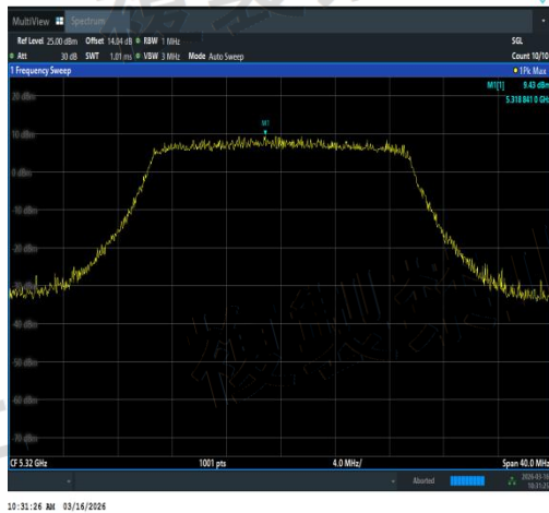
NTVN-11AX20MIMO-Ant1-5320-TPC_H-PASS
