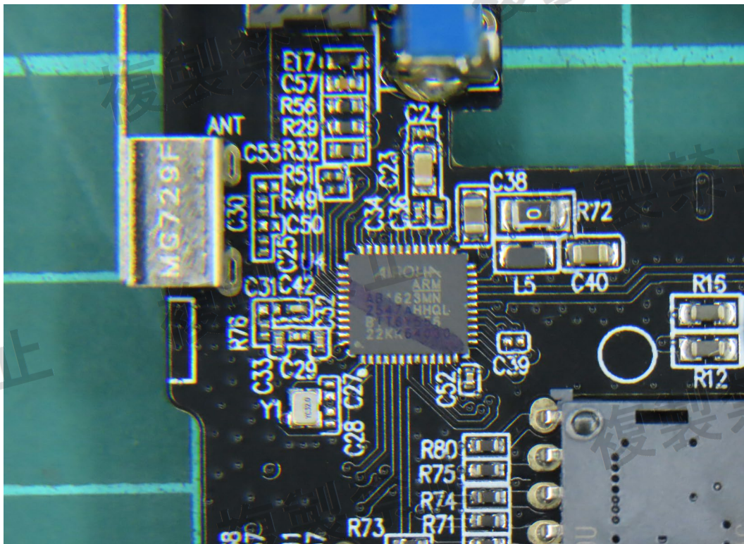
(26) EUT Photo
