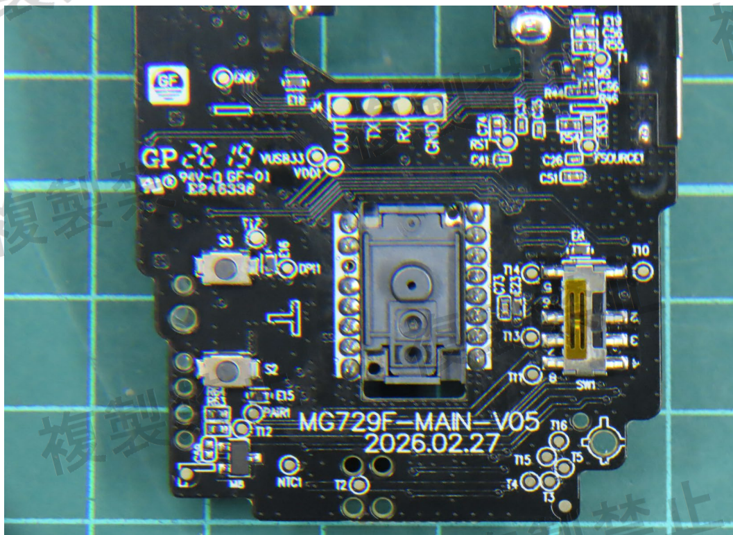
(32) EUT Photo
