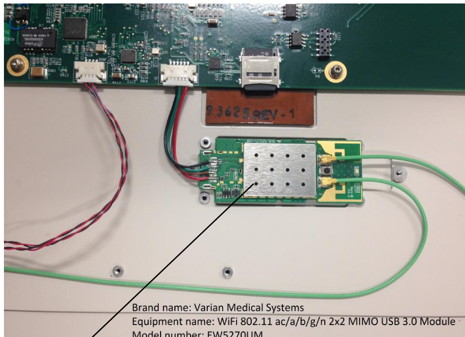
Photo 1: Module appearance
