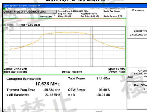
Ch.13: 2 472MHz
