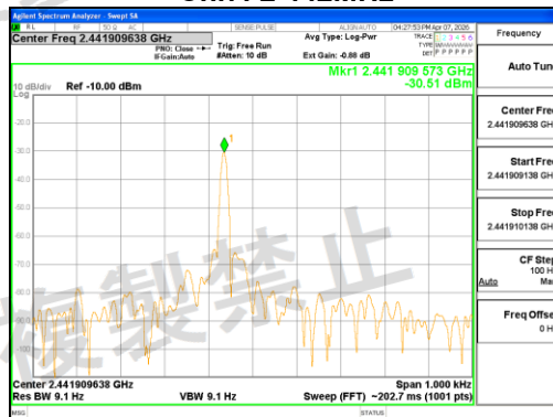
Ch.7: 2 442MHz
