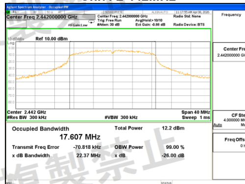
Ch.7: 2 442MHz
