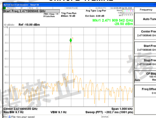
Ch.13: 2 472MHz
