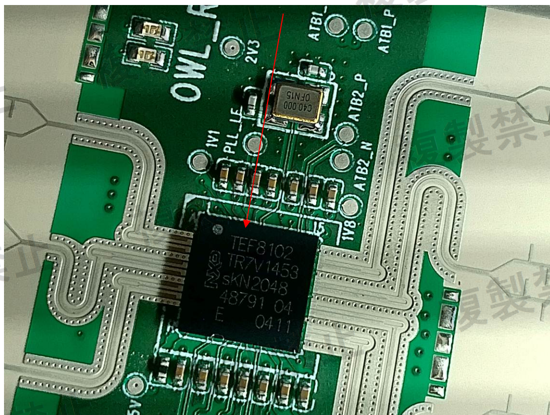
TX 2 Chip
