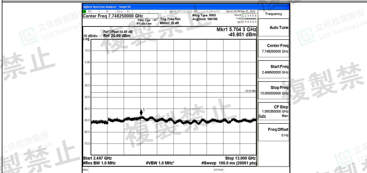
NTNV_11B_Ant1_2472_2496.5~13000
