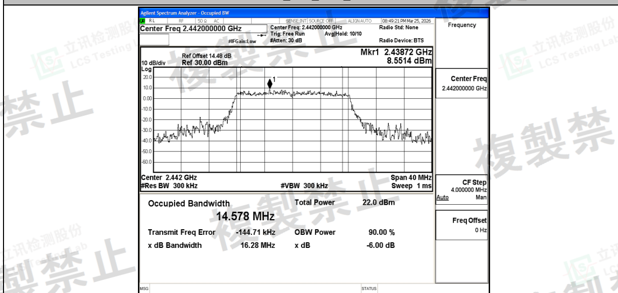
NTNV_11G_Ant1_2442
