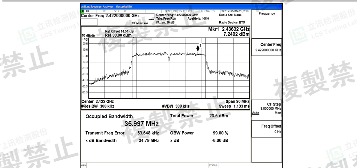
NTNV_11N40SISO_Ant1_2422
