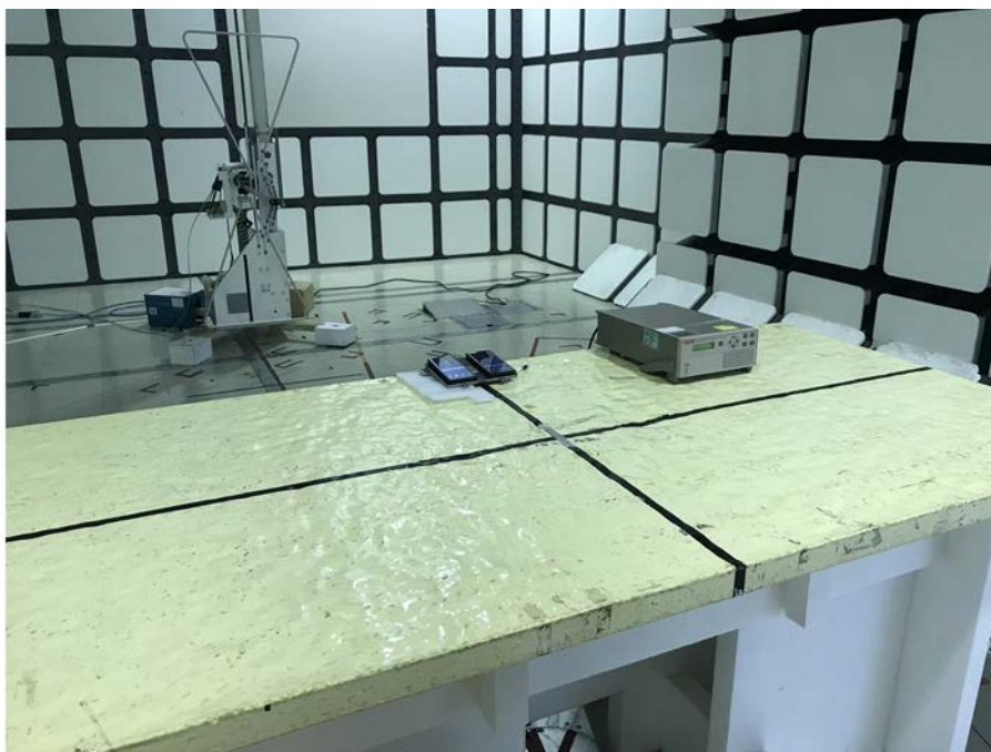
30 MHz ~ 1 GHz _ Rear View
