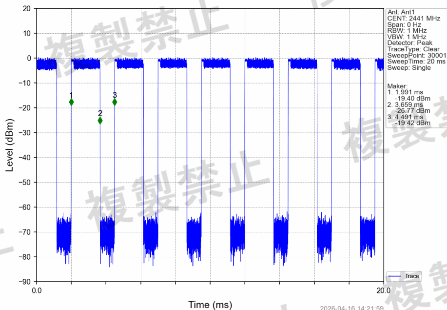
8DPSK_3DH3_2441MHz_Ant1_NTHV
